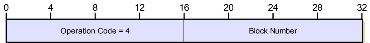
Figure 298: TFTP Acknowledgment Message Format
