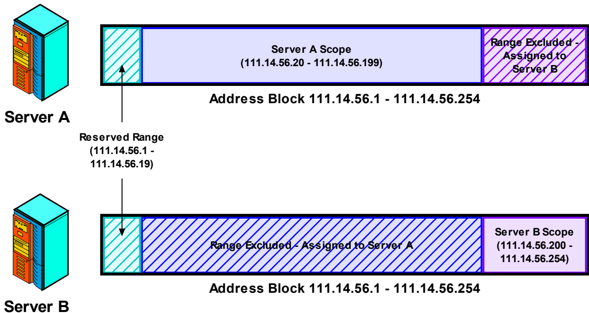
Figure 261: DHCP Multi-Server Non-Overlapping Scopes
