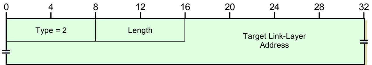
Figure 165: ICMPv6 Target Link-Layer Address Option Format
