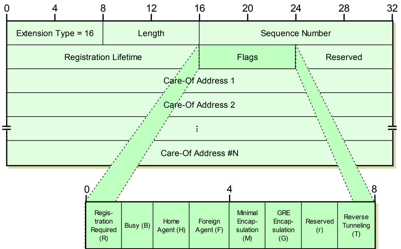
Figure 130: Mobile IP Mobility Agent Advertisement Extension Format
