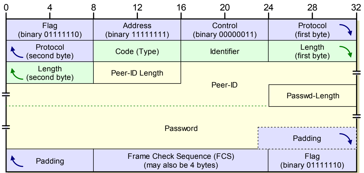
Figure 37: PPP PAP Authenticate-Request Frame Format
