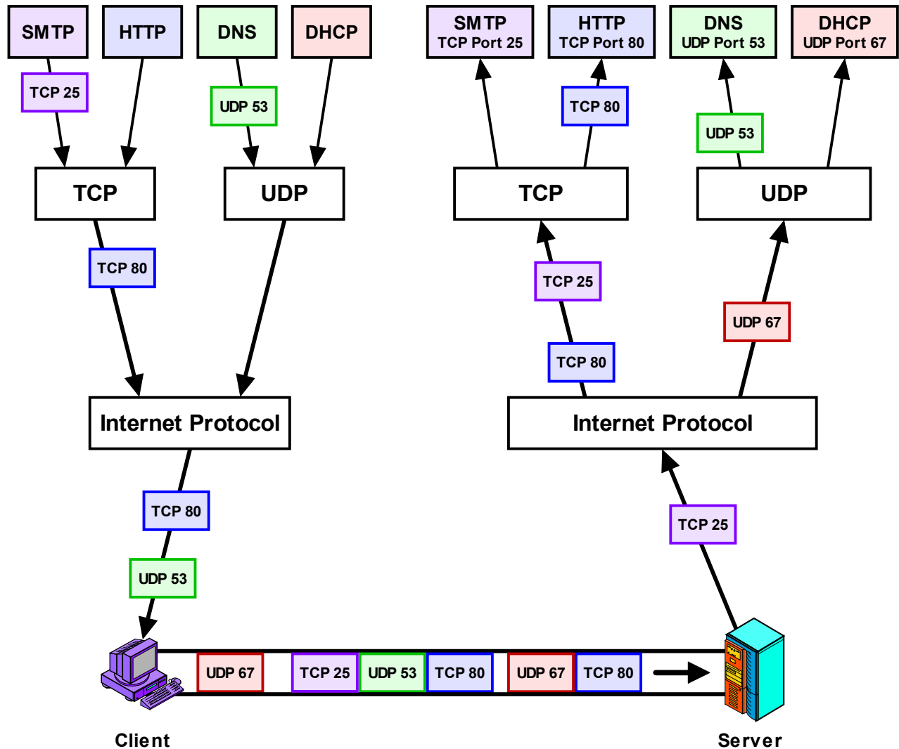
Figure 198: TCP/IP Process Multiplexing/Demultiplexing Using TCP/UDP Ports
