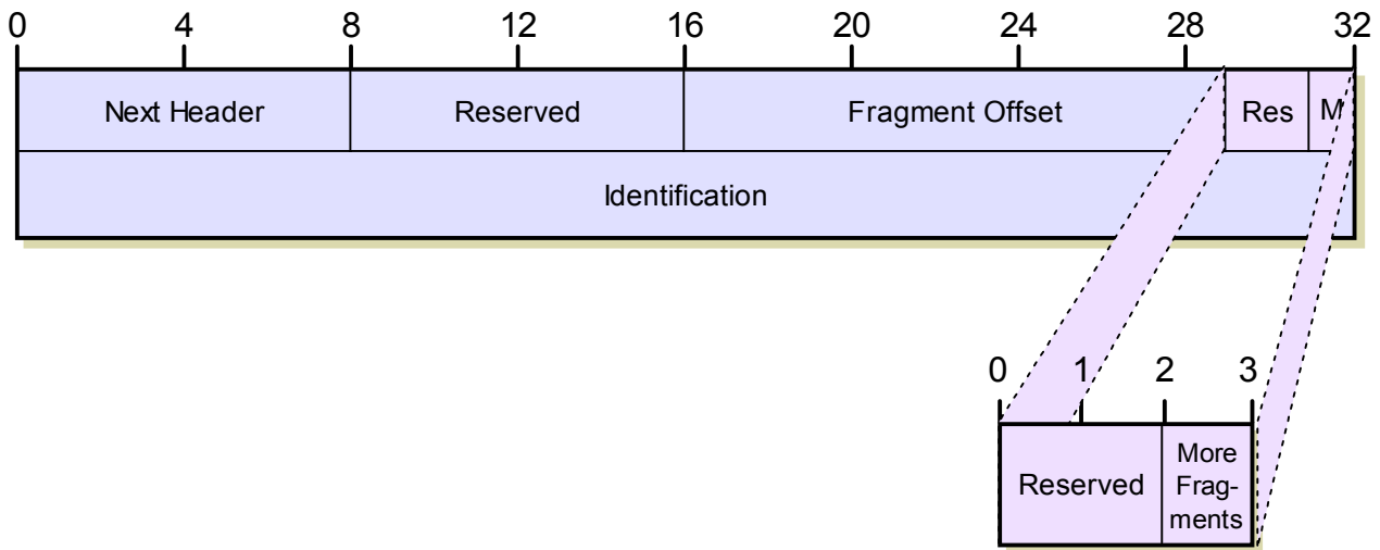
Figure 108: IPv6 Fragment Extension Header Format
