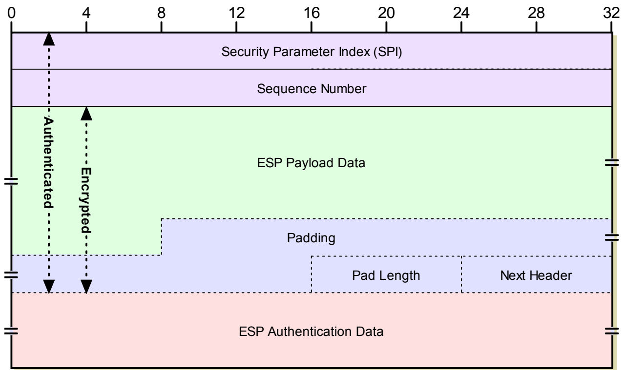
Figure 126: IPsec Encapsulating Security Payload (ESP) Format
