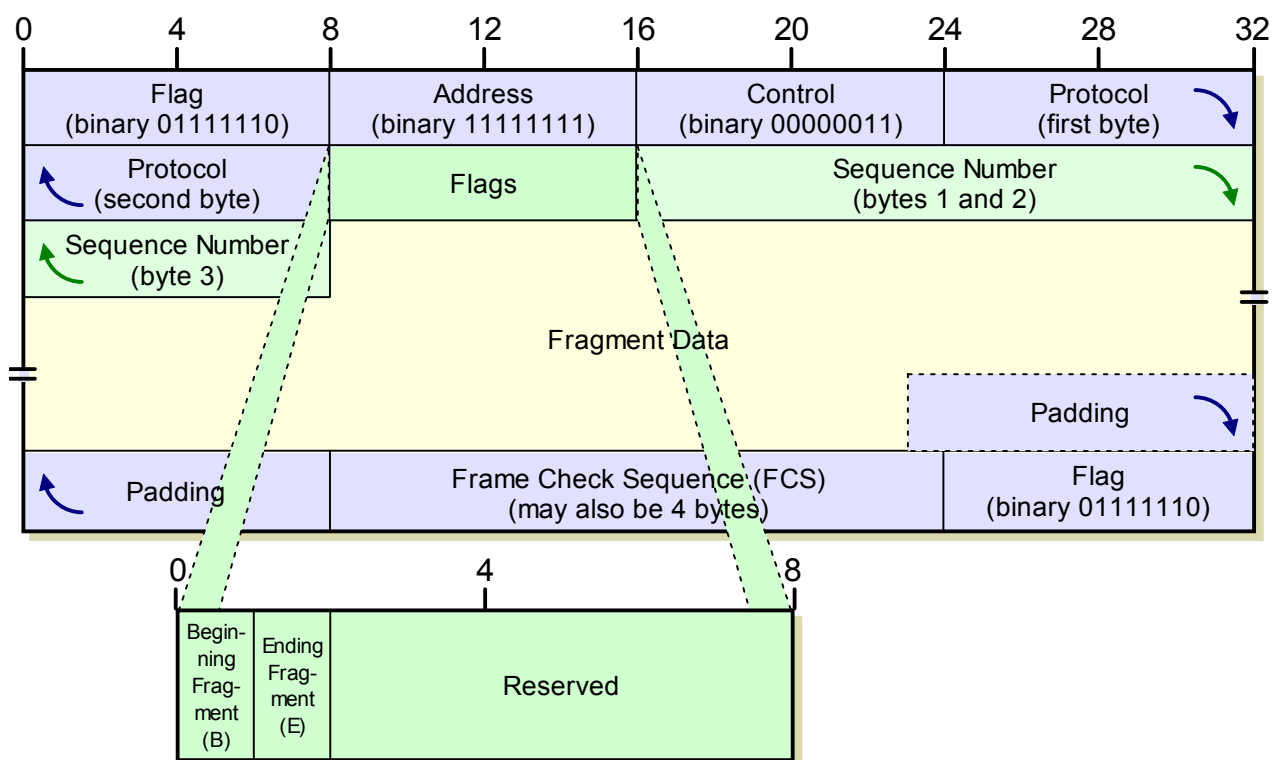
Figure 41: PPP Multilink Protocol Long Fragment Frame Format
