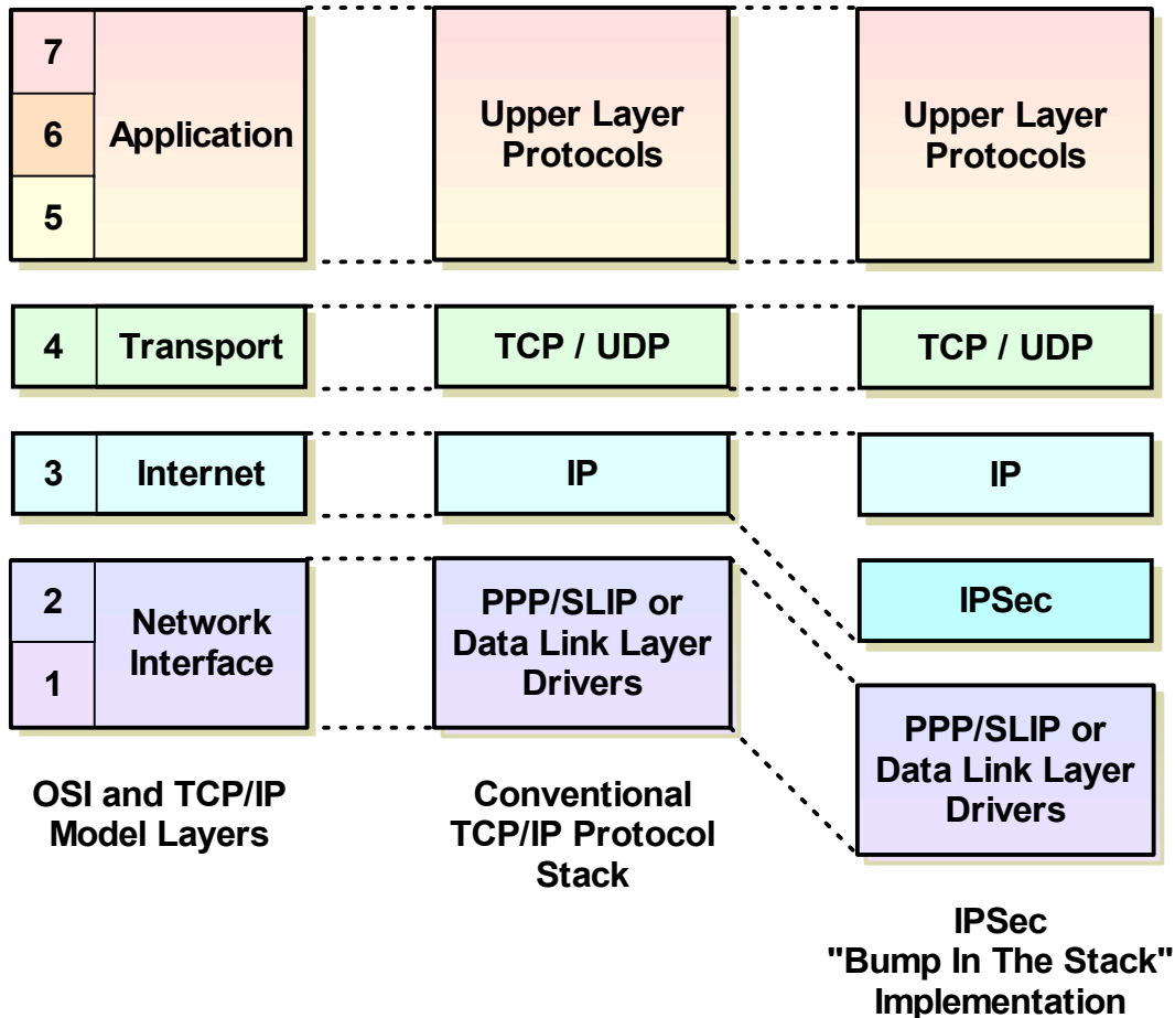
Figure 117: IPSec “Bump In The Stack” (BITS) Architecture
