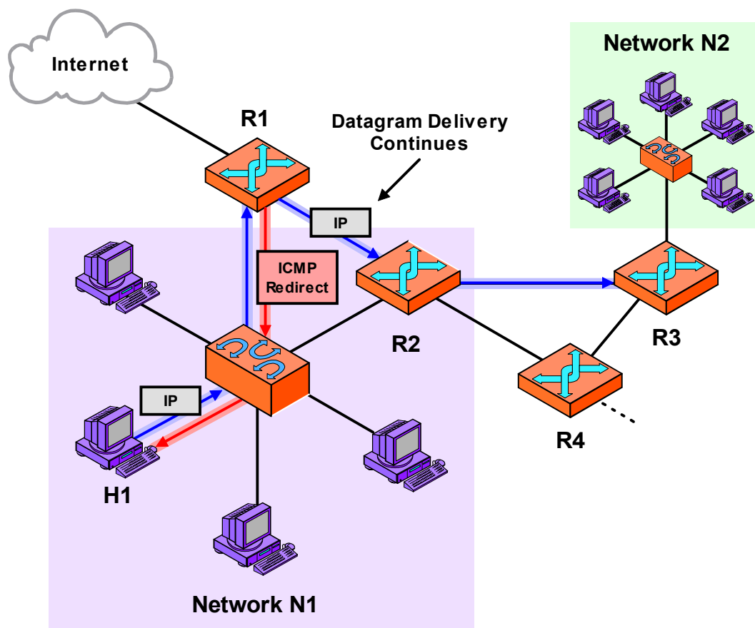
Figure 143: Host Redirection Using an ICMP Redirect Message
