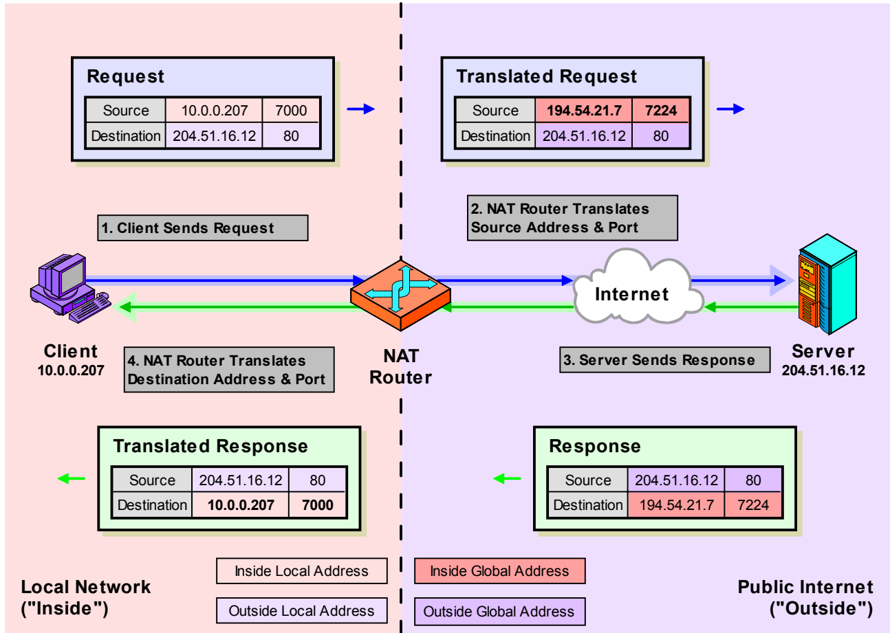
Figure 114: Operation Of Port-Based (“Overloaded”) NAT
