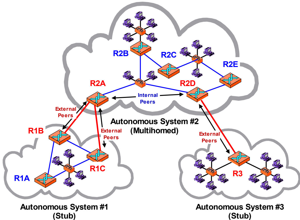
Figure 191: BGP Example Topology and Designations
