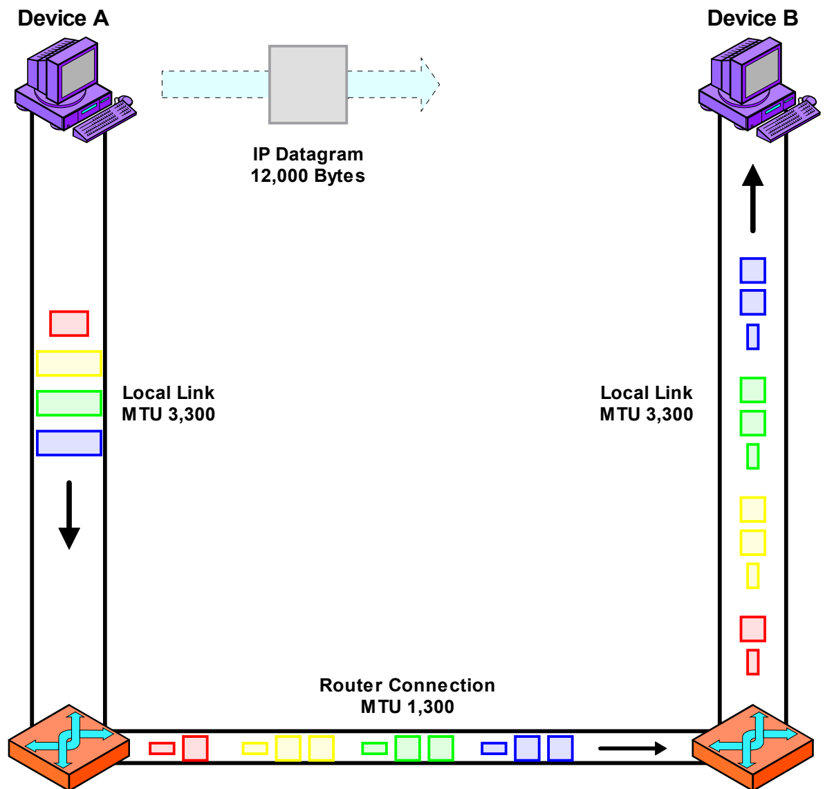
Figure 89: IPv4 Datagram Fragmentation
