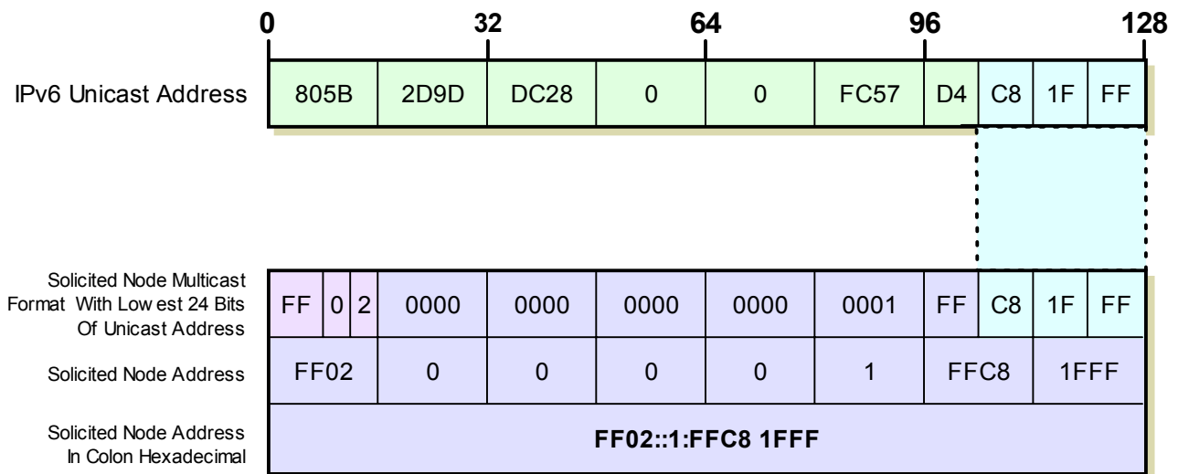
Figure 103: IPv6 Solicited Node Address Calculation
