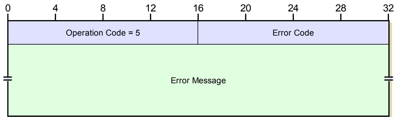
Figure 299: TFTP Error Message Format
