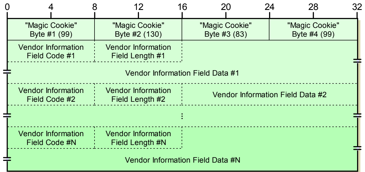
Figure 257: BOOTP Vendor-Specific Area Format Showing Vendor Information Fields
