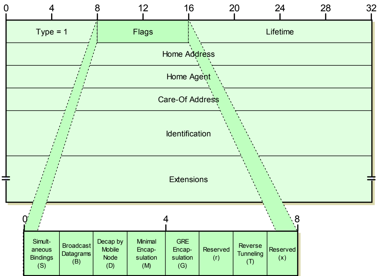
Figure 132: Mobile IP Registration Request Message Format
