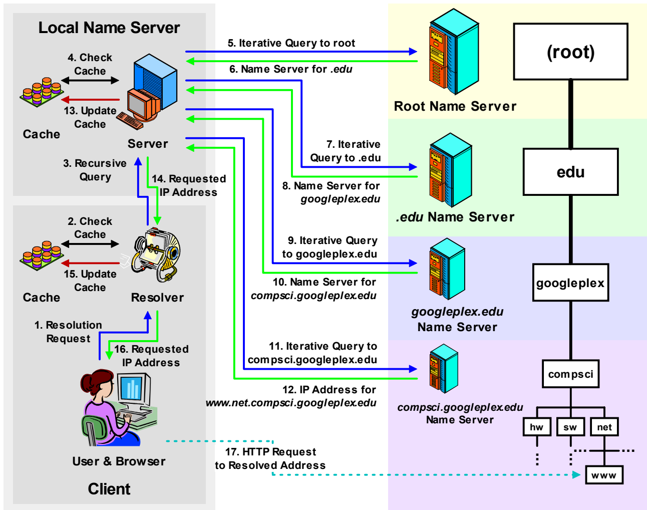
Figure 245: Example Of The DNS Name Resolution Process
