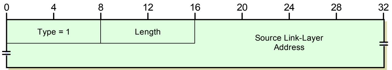
Figure 164: ICMPv6 Source Link-Layer Address Option Format
