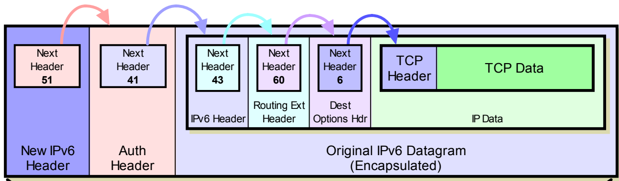
IPv6 AH Datagram Format - IPsec Transport Mode
