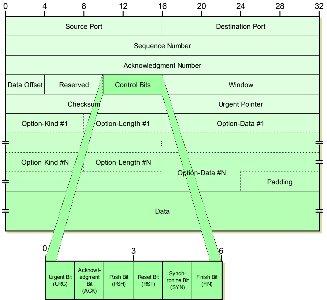
Figure 216: TCP Segment Format
