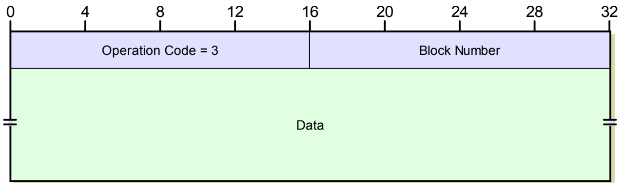
Figure 297: TFTP Data Message Format
