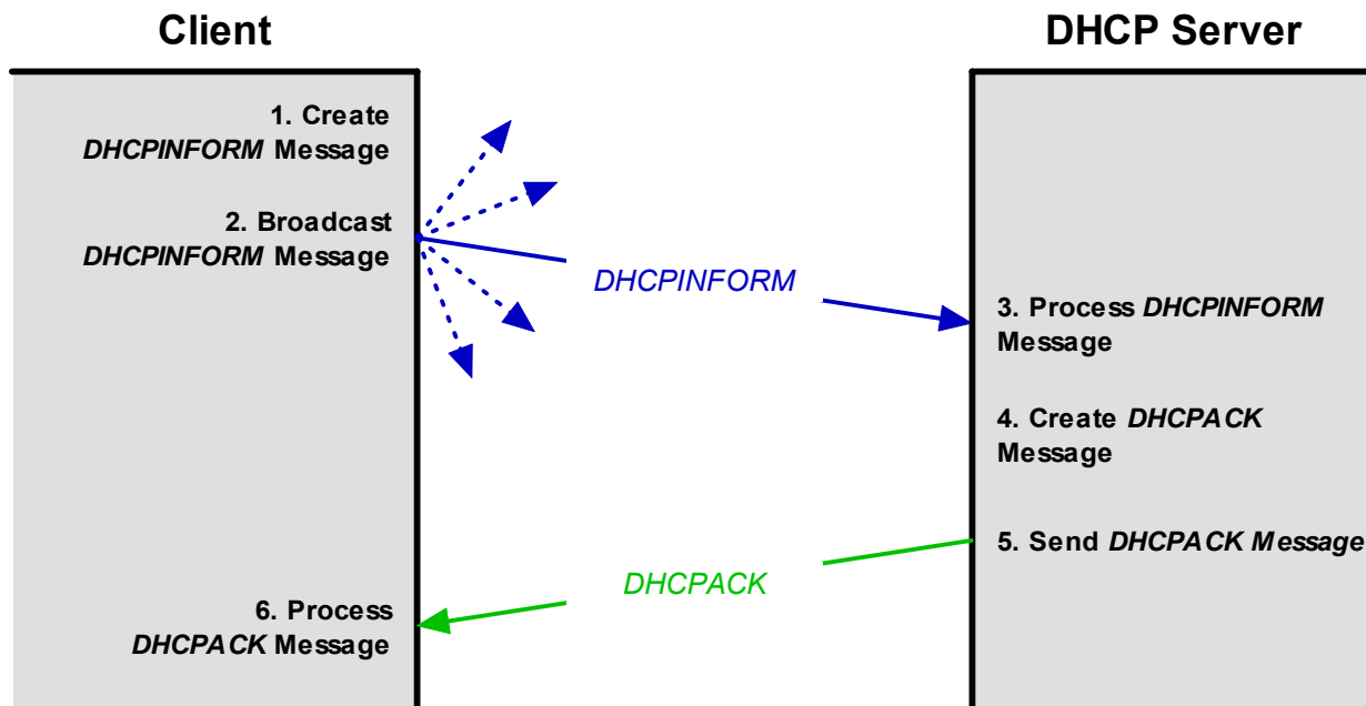
Figure 266: DHCP Parameter Configuration Process
