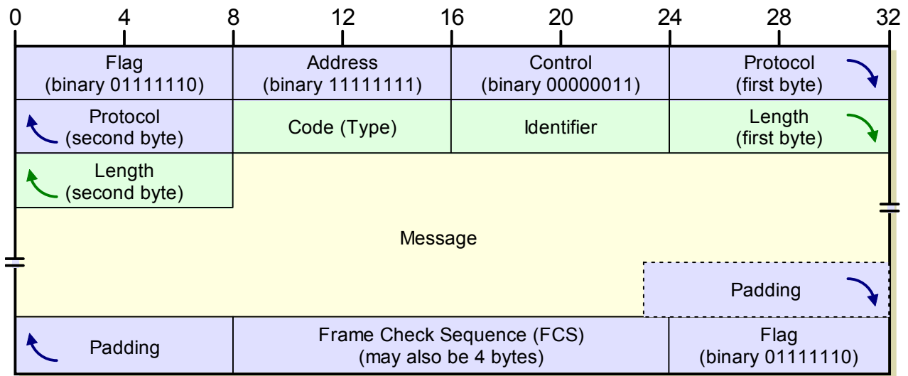
Figure 40: PPP CHAP Success and Failure Frame Format
