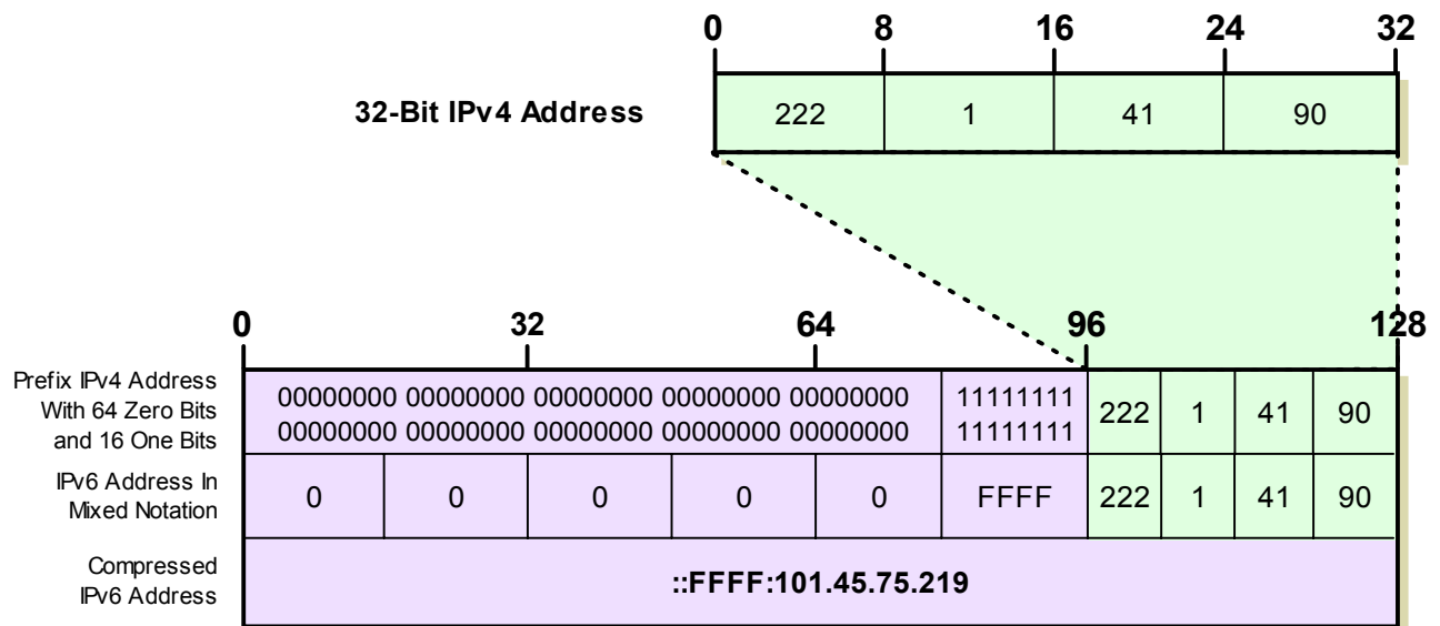
Figure 100: IPv4-Mapped Embedded IPv6 Address Representation
