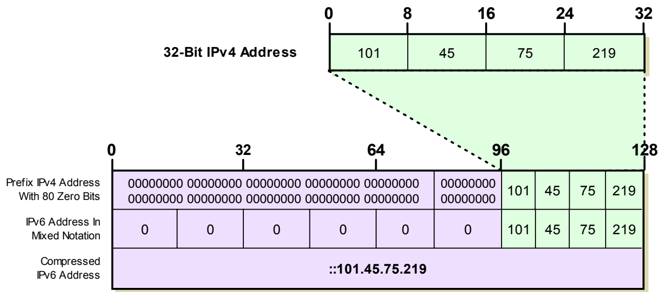
Figure 99: IPv4-Compatible Embedded IPv6 Address Representation
