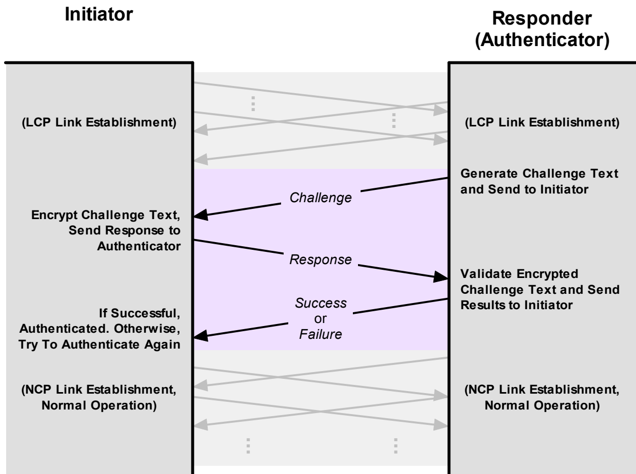
Figure 30: PPP Challenge Handshake Authentication Protocol (CHAP) Authentication
