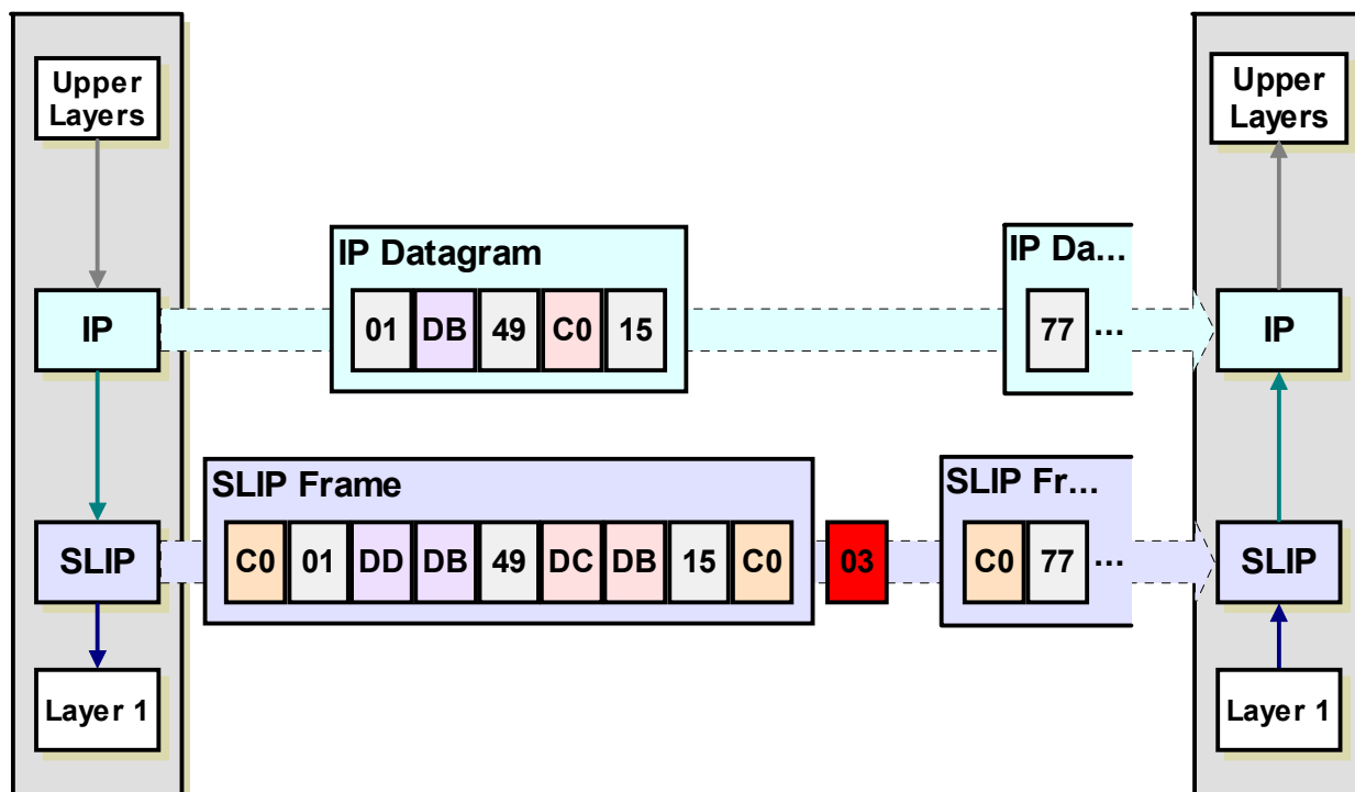
Figure 22: Operation of the Serial Line Internet Protocol (SLIP)
