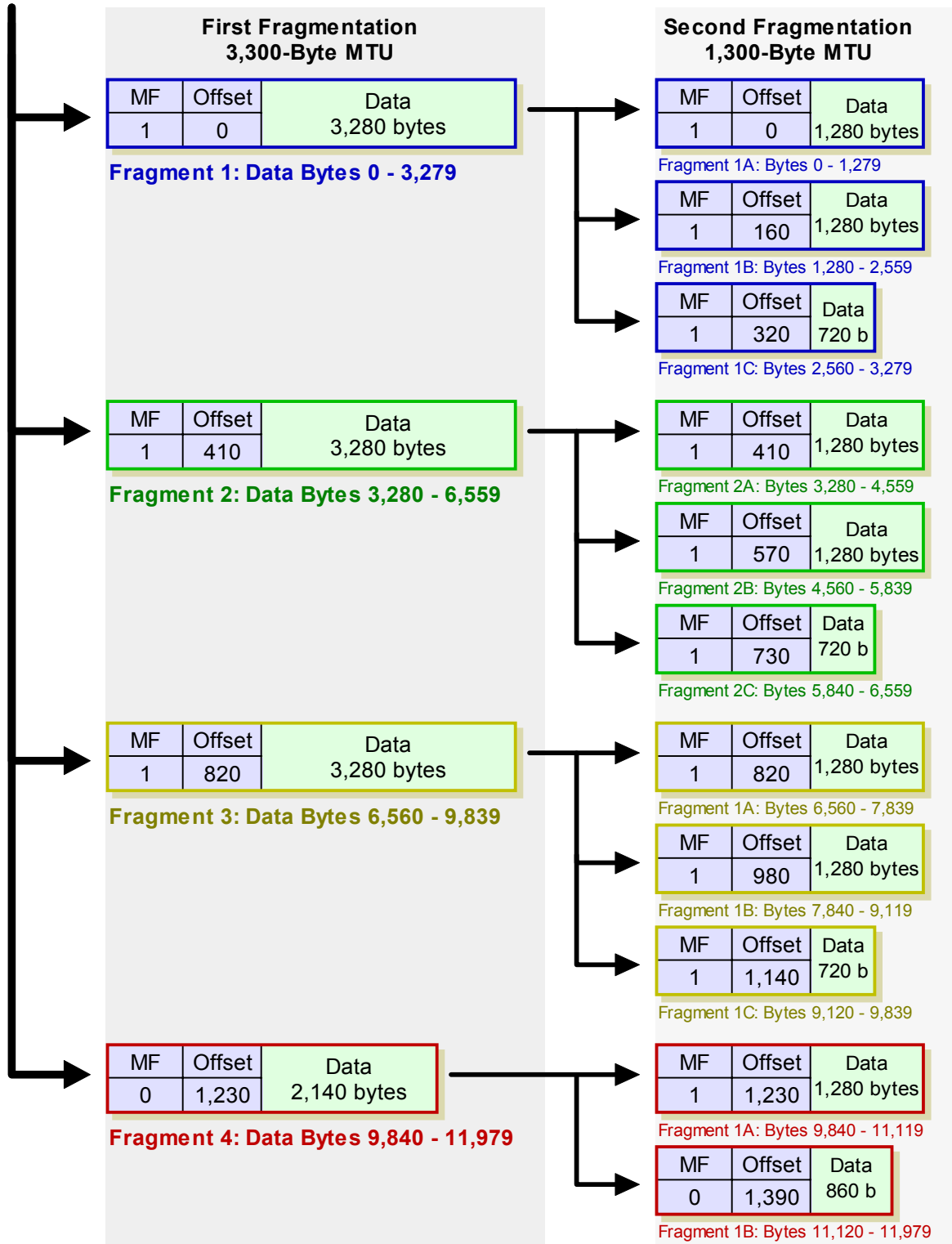
Figure 90: IPv4 Datagram Fragmentation Process
