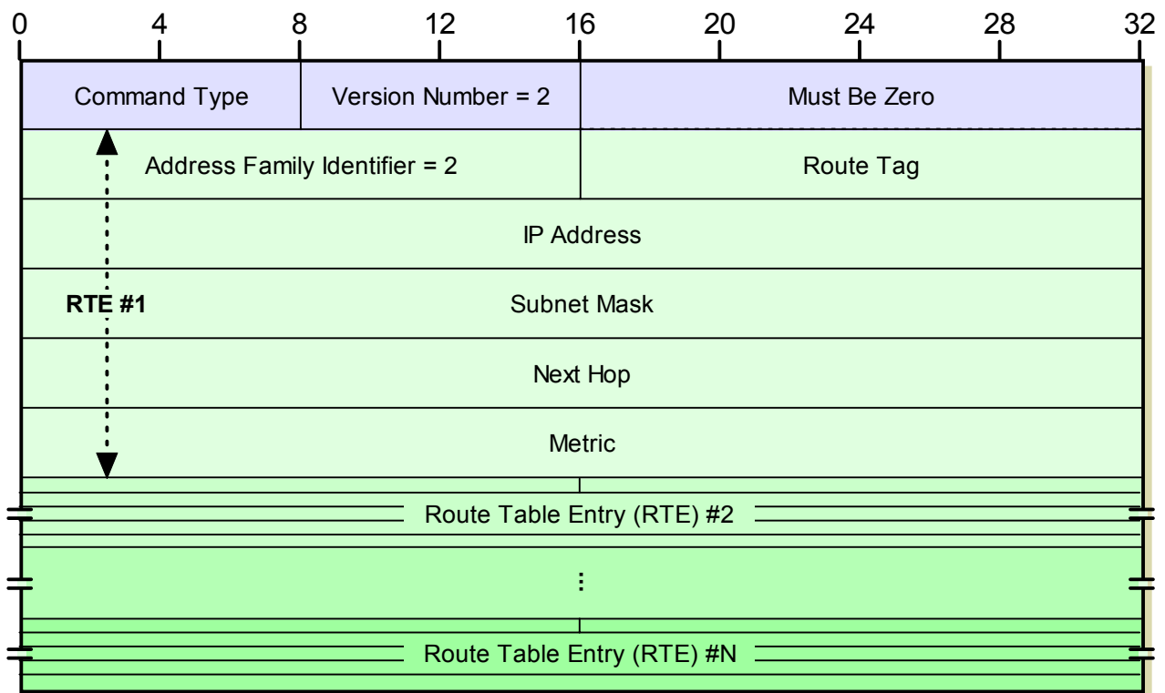
Figure 177: RIP Version 2 (RIP-2) Message Format
