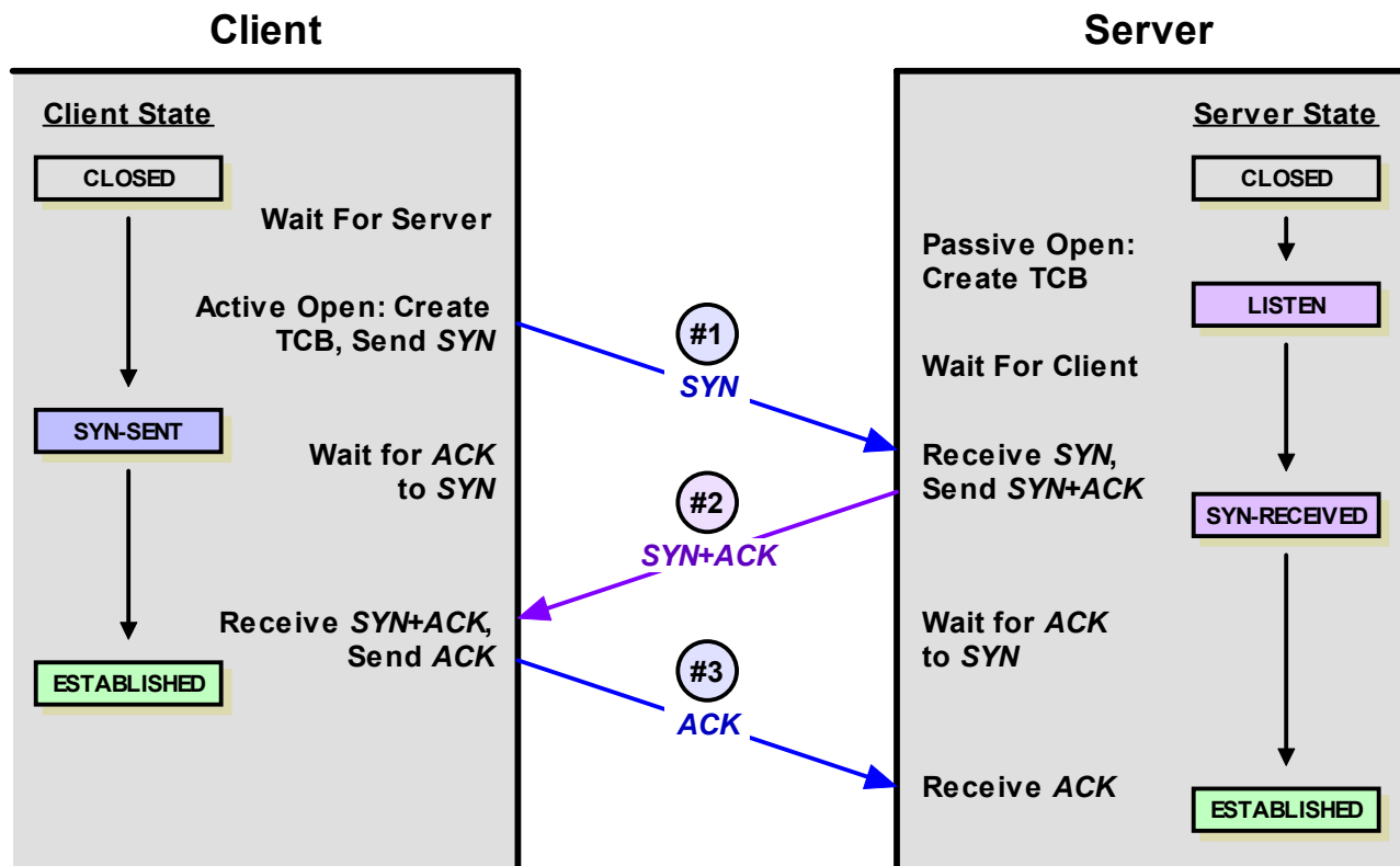
Figure 211: TCP “Three-Way Handshake” Connection Establishment Procedure
