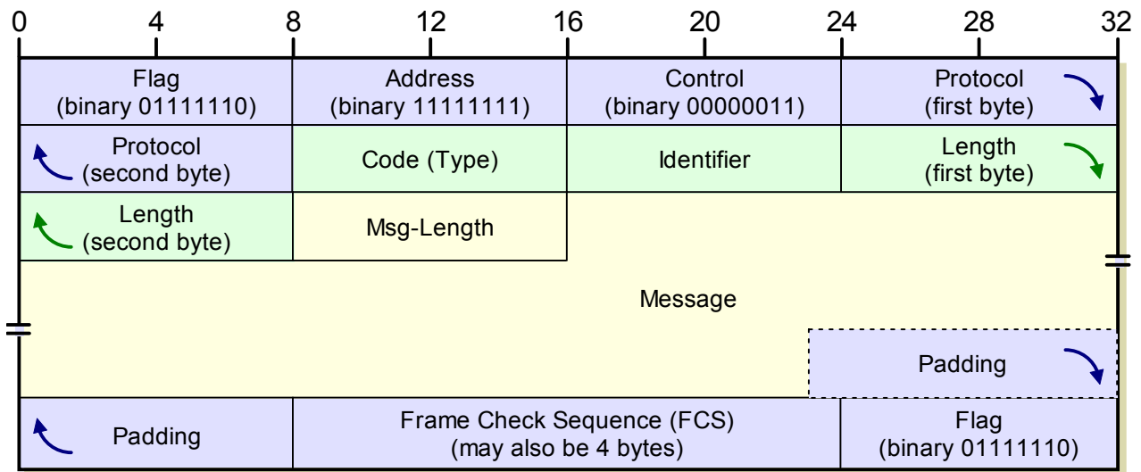
Figure 38: PPP PAP Authenticate-Ack and Authenticate-Nak Frame Format
