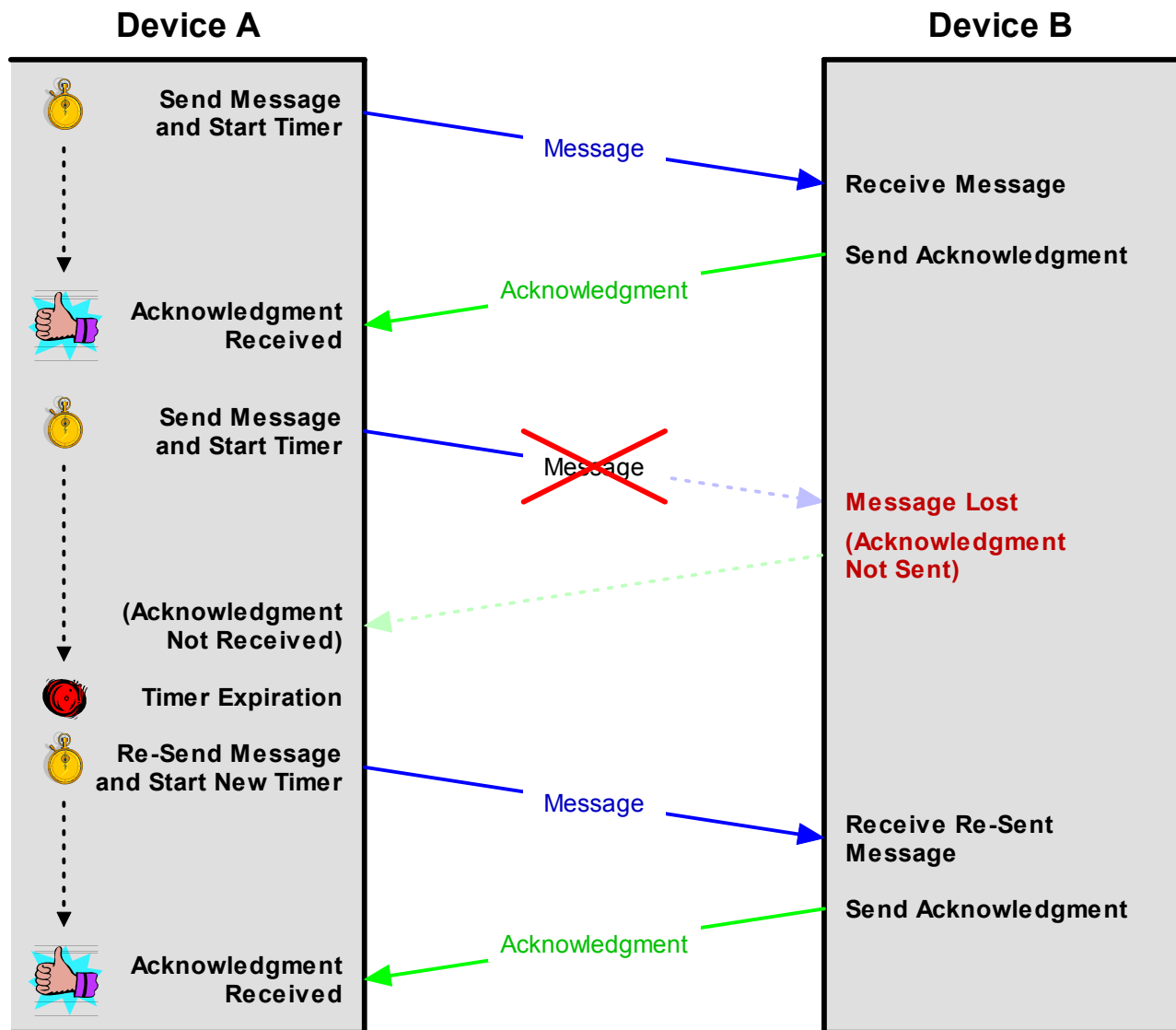
Figure 204: Basic Reliability: Positive Acknowledgment With Retransmission (PAR)
