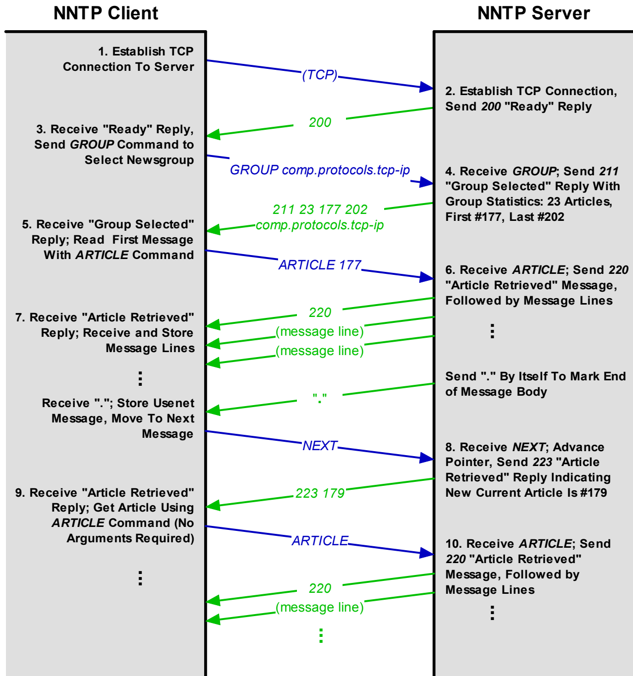
Figure 313: NNTP Full Newsgroup Retrieval Process
