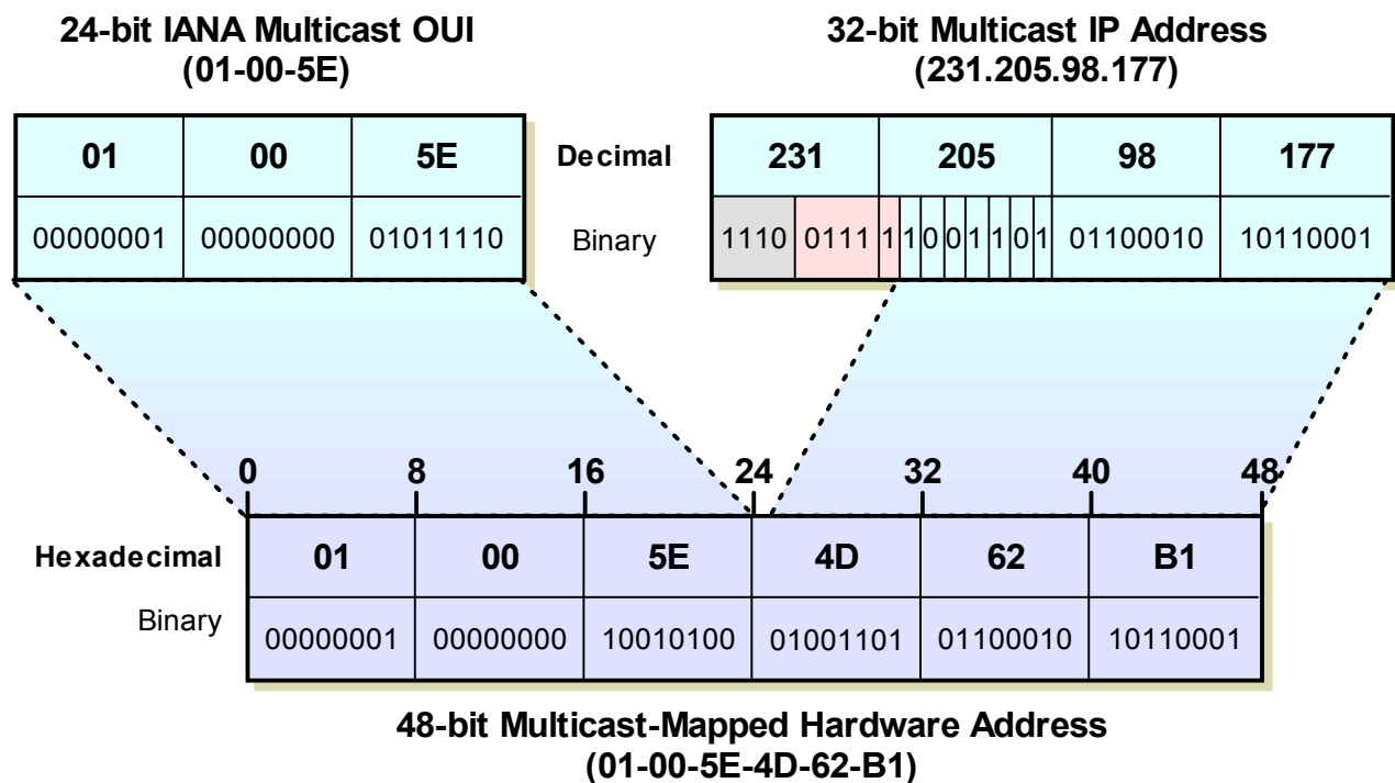
Figure 51: Mapping of Multicast IP Addresses to IEEE 802 Multicast MAC Addresses IP multicast addresses consist of the bit string “1110” followed by a 28-bit multicast group address. To create a 48-bit multicast IEEE 802 (Ethernet) address, the top 24 bits are filled in with the IANA’s multicast OUI, 01-00-5E, the 25th bit is zero, and the bottom 23 bits of the multicast group are put into the bottom 23 bits of the MAC address. This leaves 5 bits (shown in pink) that are not mapped to the MAC address, meaning that 32 different IP addresses may have the same mapped multicast MAC address.
