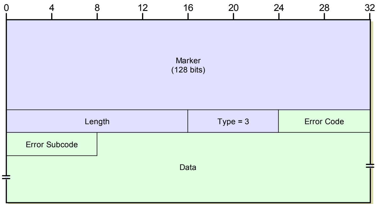
Figure 196: BGP Notification Message Format
