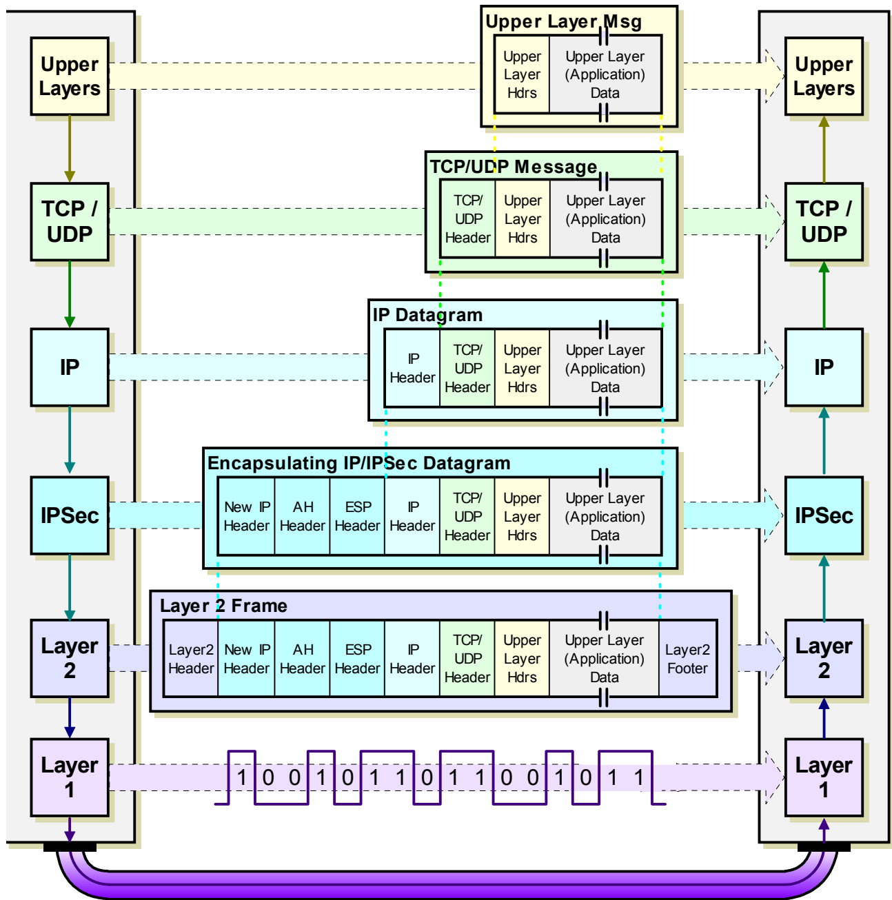
Figure 120: IPsec Tunnel Mode Operation
