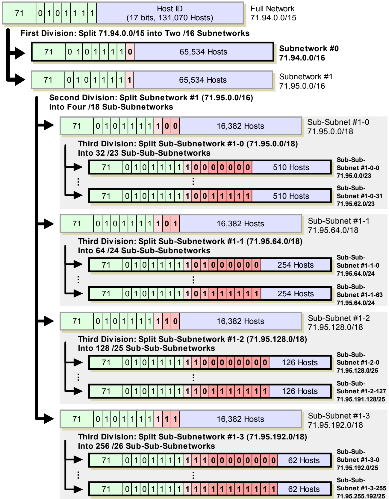
Figure 84: Hierarchical Address Division Using Classless Addressing (CIDR)
