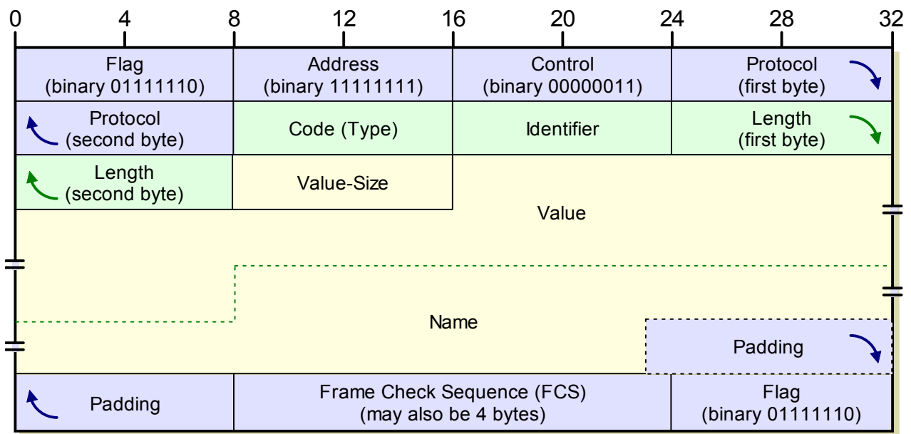
Figure 39: PPP CHAP Challenge and Response Frame Format
