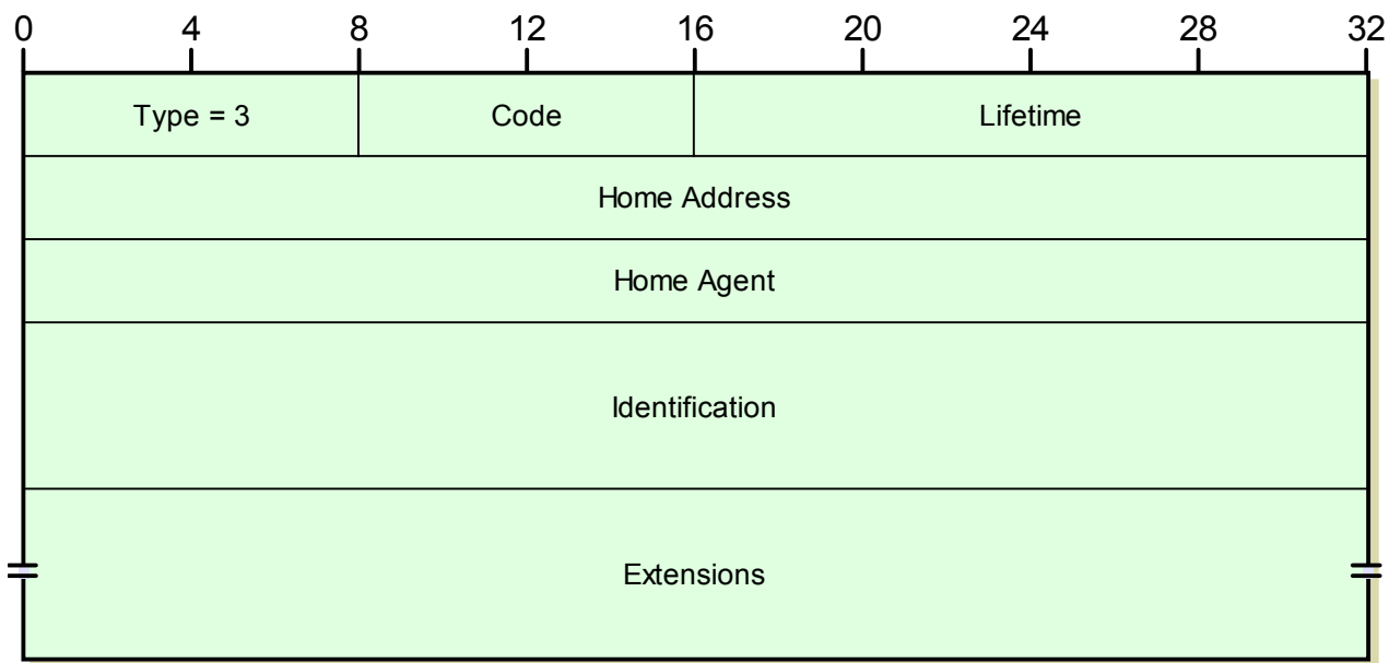
Figure 133: Mobile IP Registration Reply Message Format
