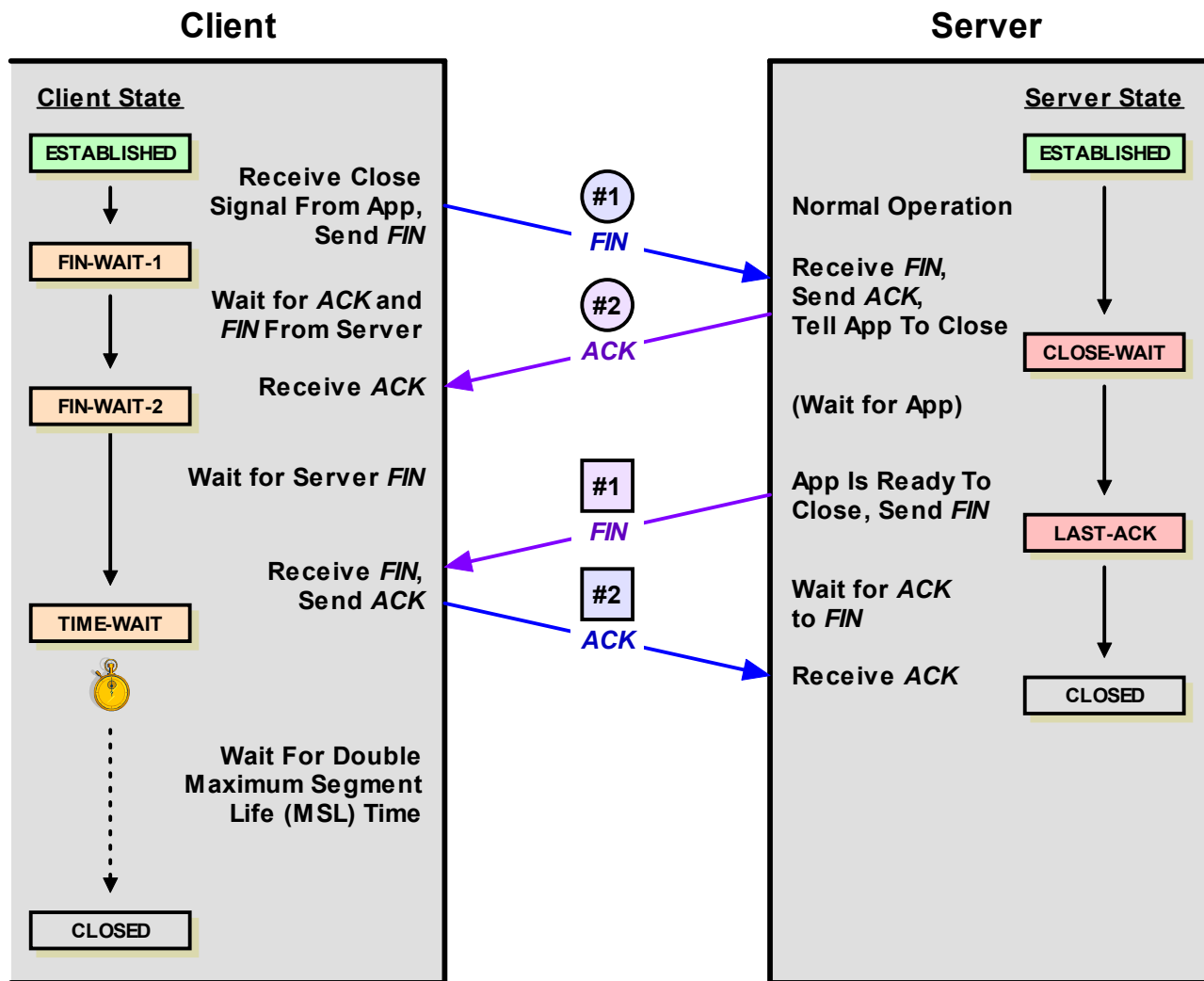
Figure 214: TCP Connection Termination Procedure
