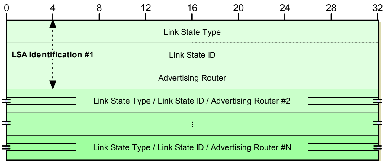
Figure 187: OSPF Link State Request Message Format
