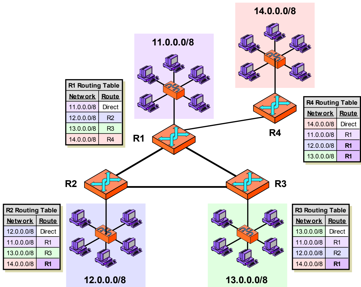
Figure 93: IP Routing and Routing Tables
