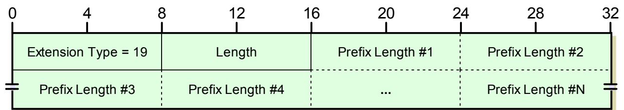
Figure 131: Mobile IP Prefix-Lengths Extension Format
