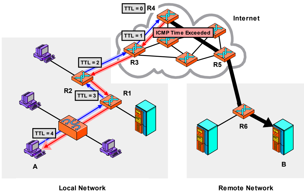
Figure 141: Expiration of an IP Datagram and Time Exceeded Message Generation
