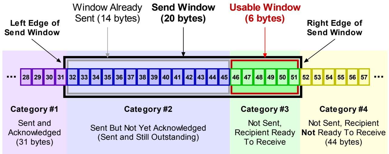
Figure 207: TCP Transmission Stream Categories and Send Window Terminology
