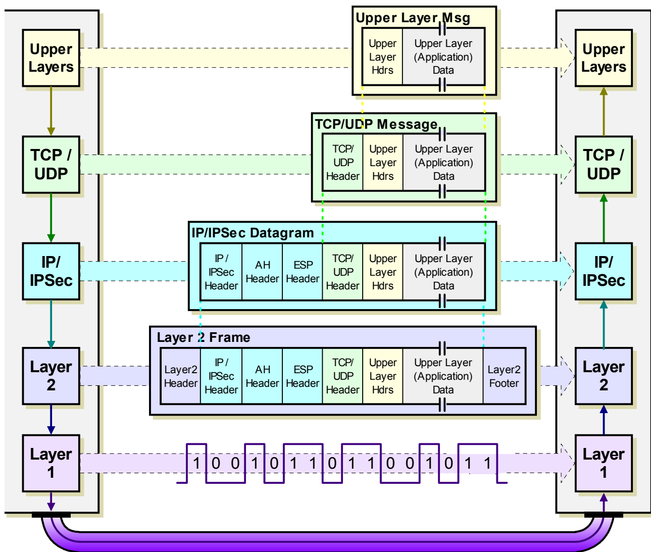
Figure 119: IPSec Transport Mode Operation
