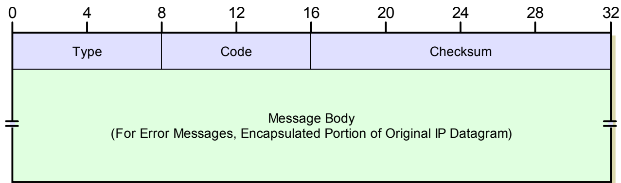
Figure 138: ICMP Common Message Format
