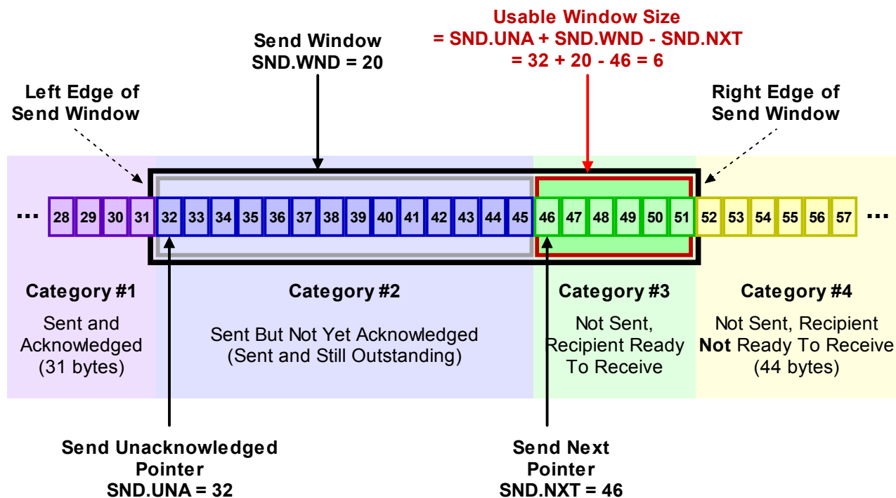
Figure 219: TCP Transmission Categories, Send Window and Pointers
