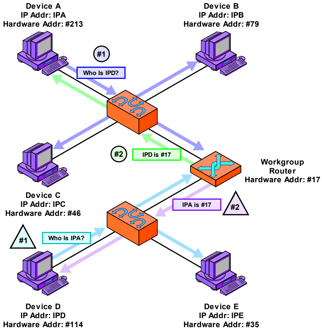
Figure 50: ARP Proxy Operation
