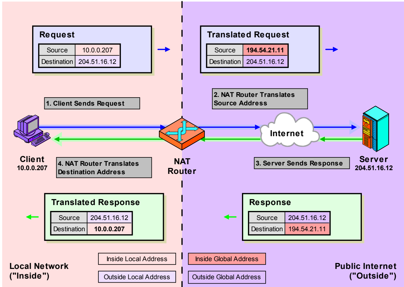
Figure 112: Operation Of Unidirectional (Traditional/Outbound) NAT
