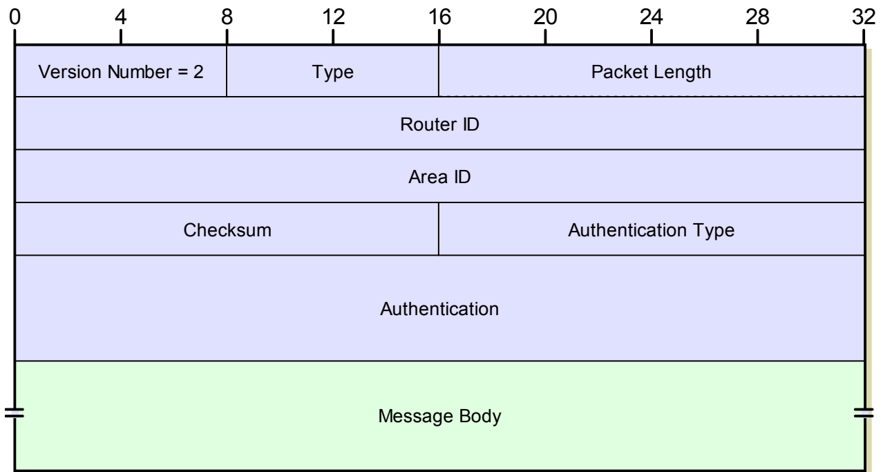
Figure 184: OSPF Common Header Format
