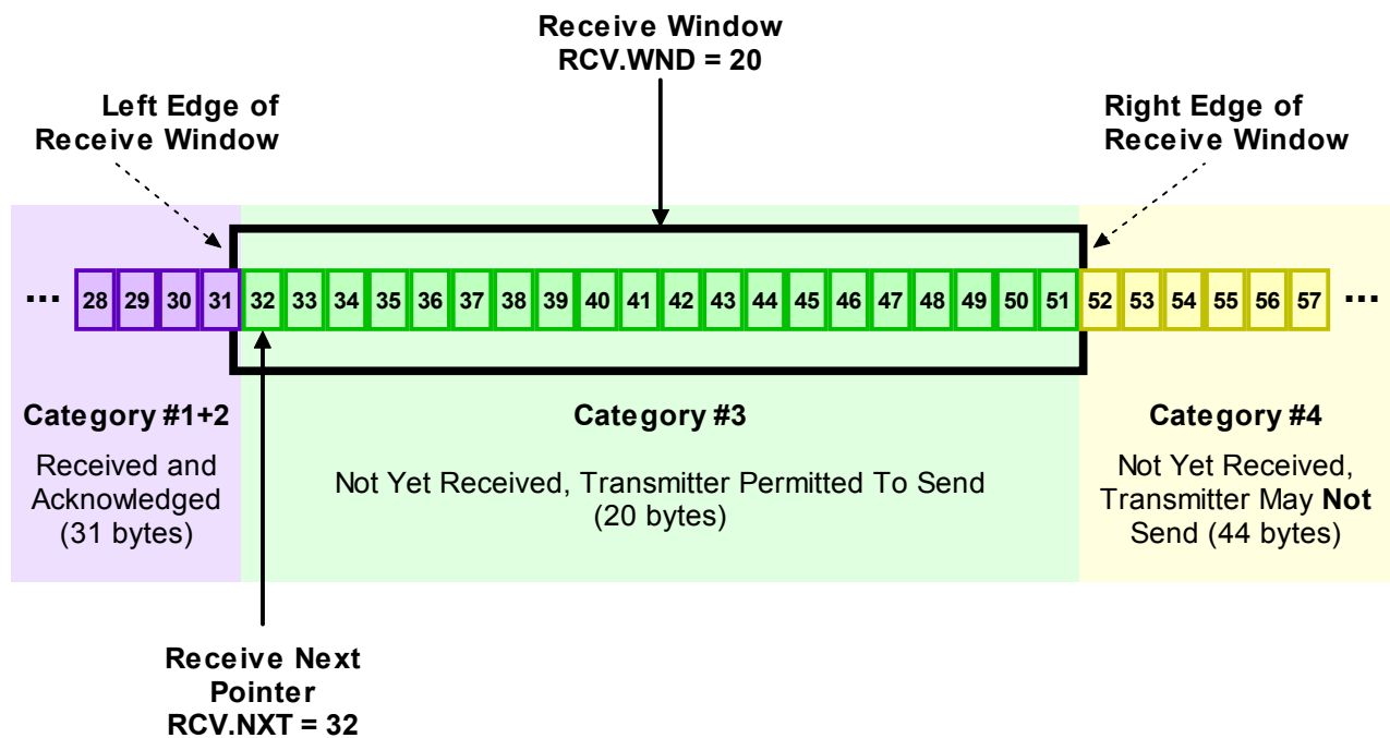
Figure 220: TCP Receive Categories and Pointers
