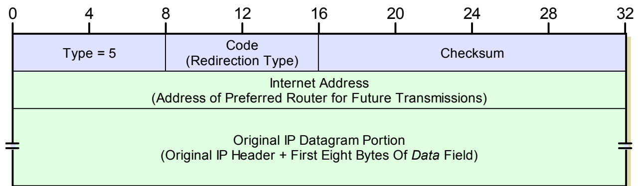
Figure 144: ICMPv4 Redirect Message Format
