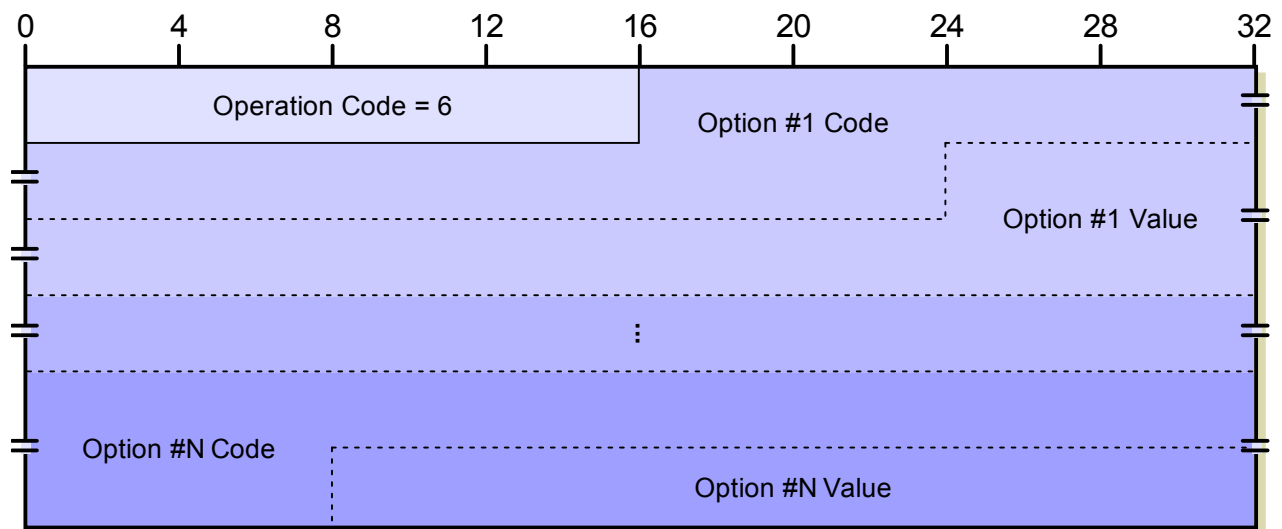
Figure 300: TFTP Option Acknowledgment Message Format
