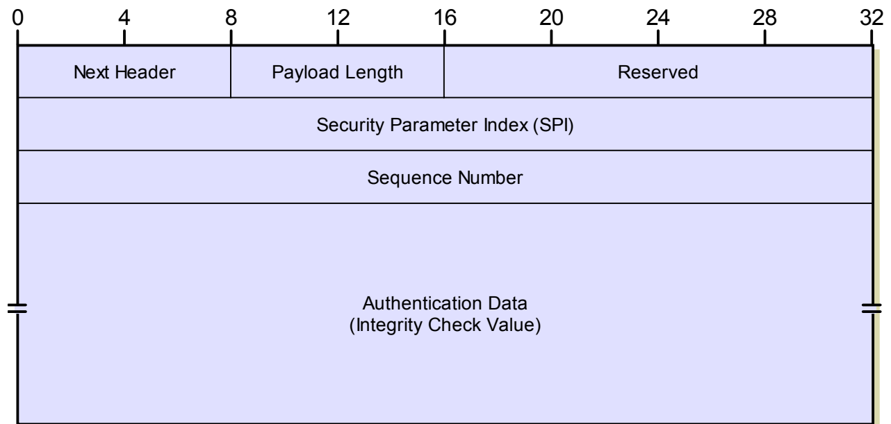
Figure 123: IPSec Authentication Header (AH) Format
