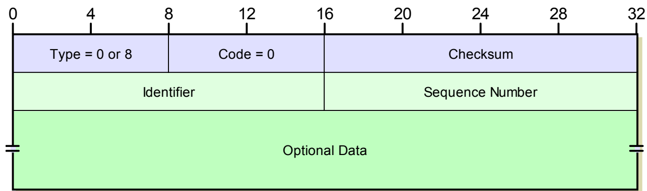
Figure 146: ICMPv4 Echo and Echo Reply Message Format
