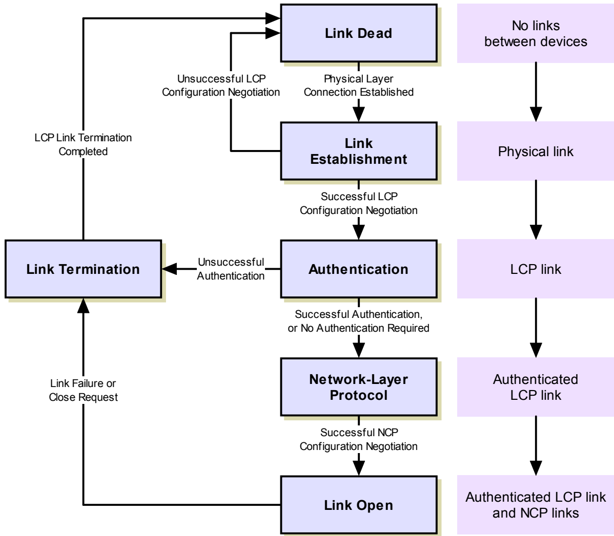
Figure 25: PPP Phases
