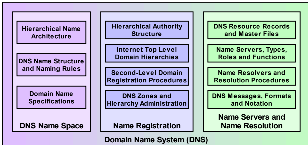
Figure 234: DNS Functions
