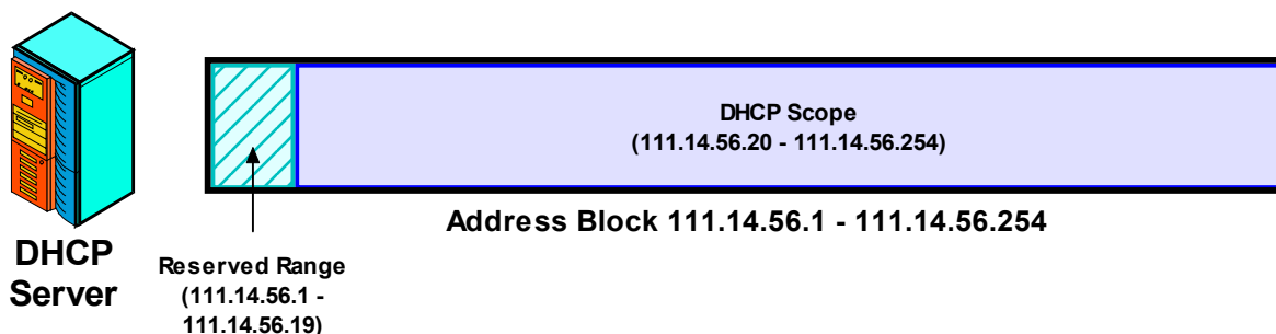
Figure 260: DHCP Scope
