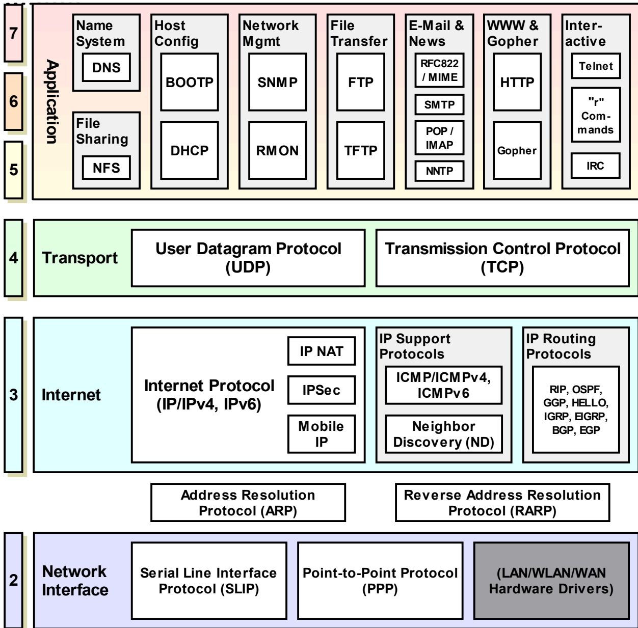
Figure 21: TCP/IP Protocols
