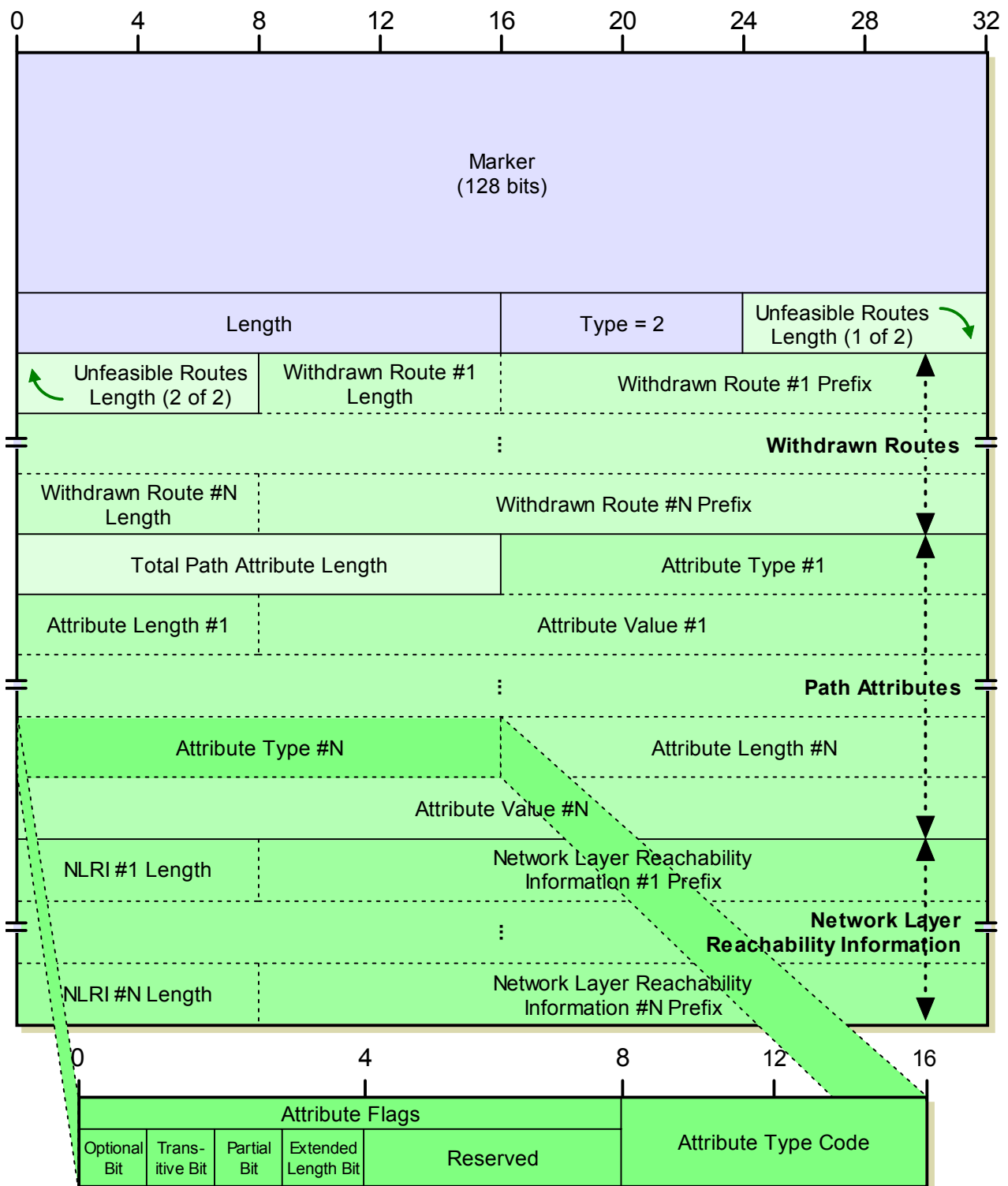
Figure 194: BGP Update Message Format
