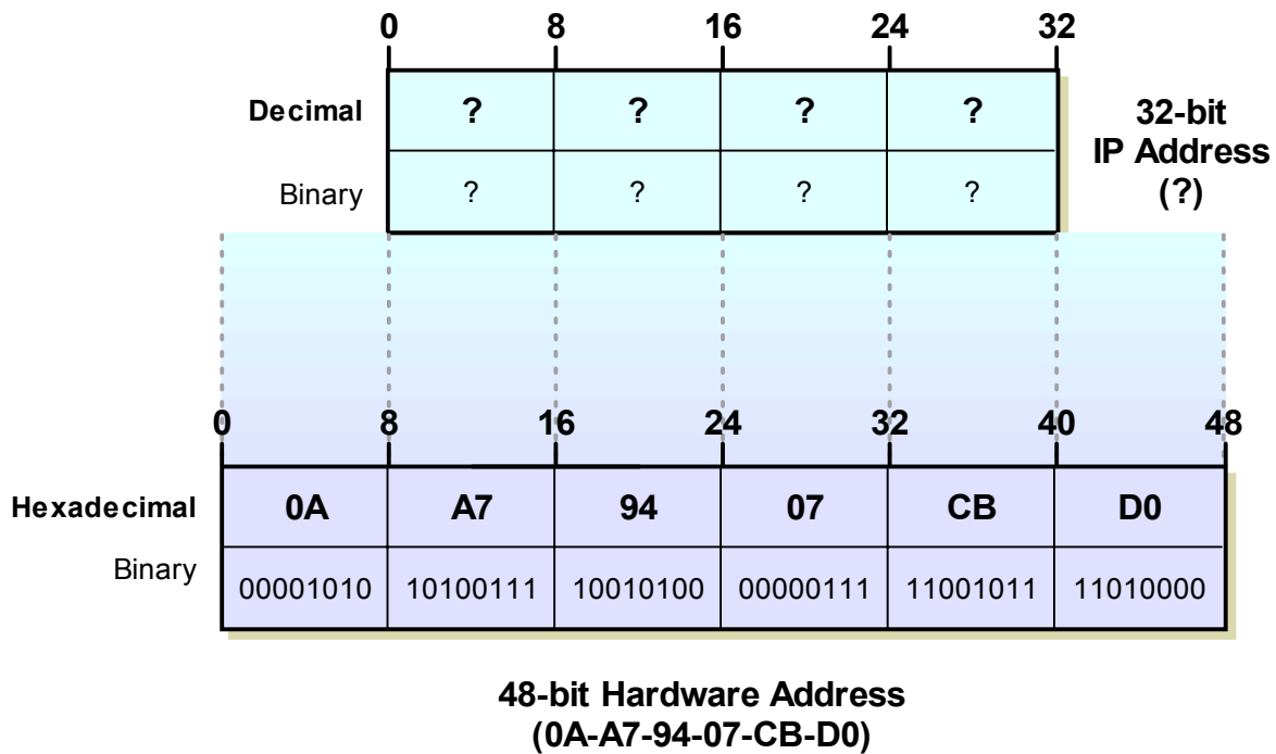
Figure 46: Address Resolution Problems With Large Hardware Address Size
