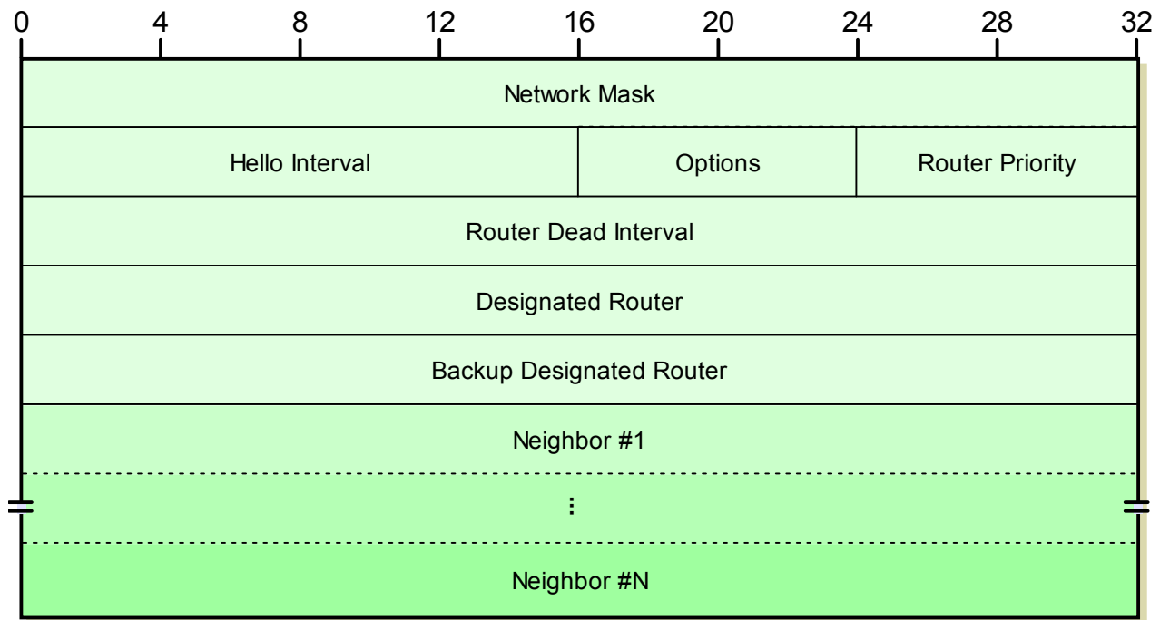
Figure 185: OSPF Hello Message Format
