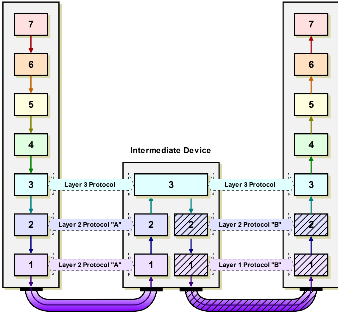
Figure 17: Message Routing in the OSI Reference Model
