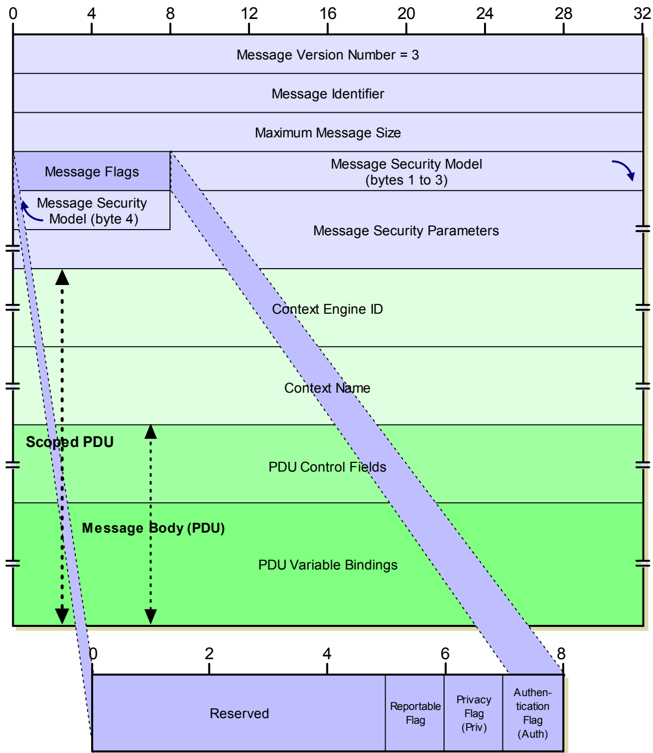
Figure 285: SNMP Version 3 (SNMPv3) General Message Format
