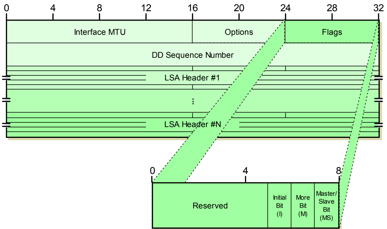
Figure 186: OSPF Database Description Message Format
