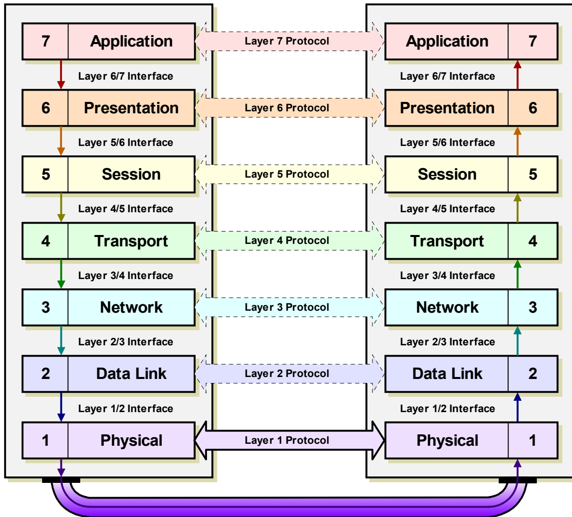
Figure 14: OSI Reference Model Protocols: Horizontal Communication
