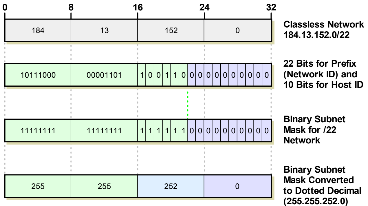
Figure 82: CIDR (“Slash”) Notation and Its Subnet Mask Equivalent
