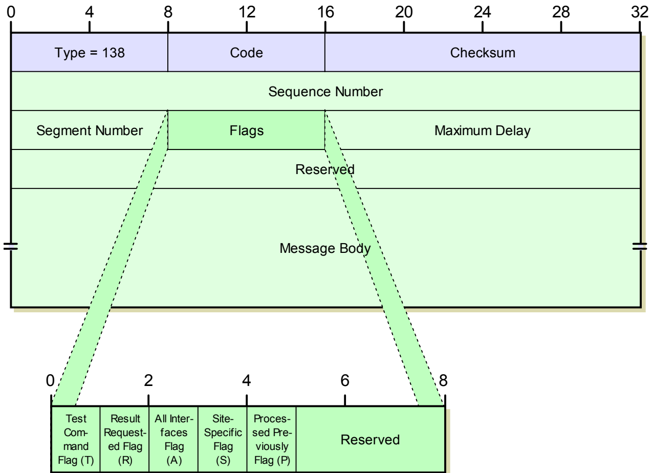
Figure 163: ICMPv6 Router Renumbering Message Format
