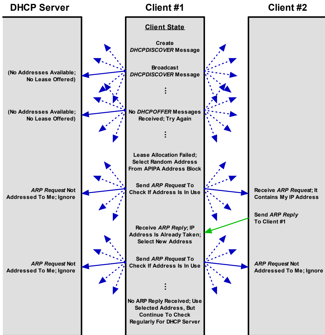
Figure 269: DHCP Automatic Private IP Addressing (APIPA)
