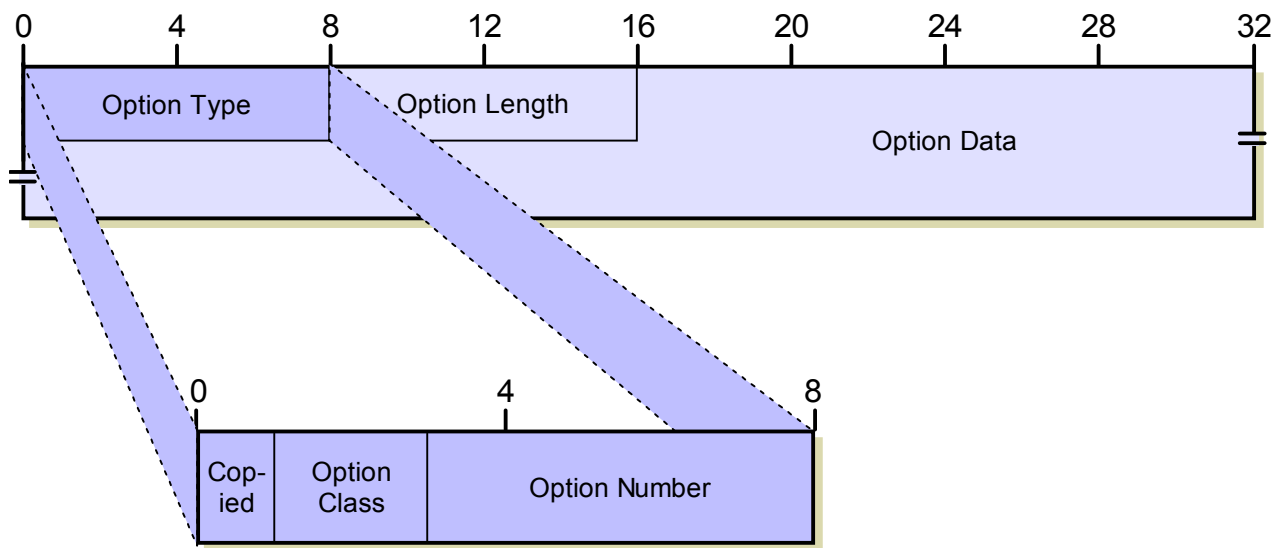
Figure 87: Internet Protocol Version 4 (IPv4) Option Format
