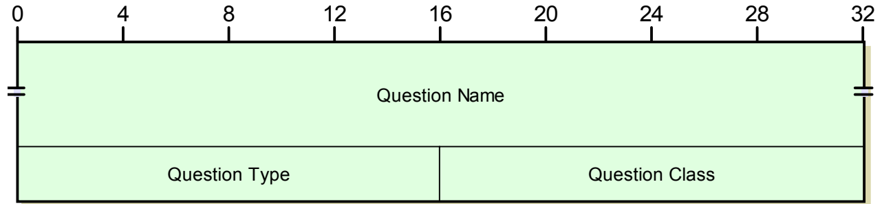
Figure 249: DNS Message Question Section Format
