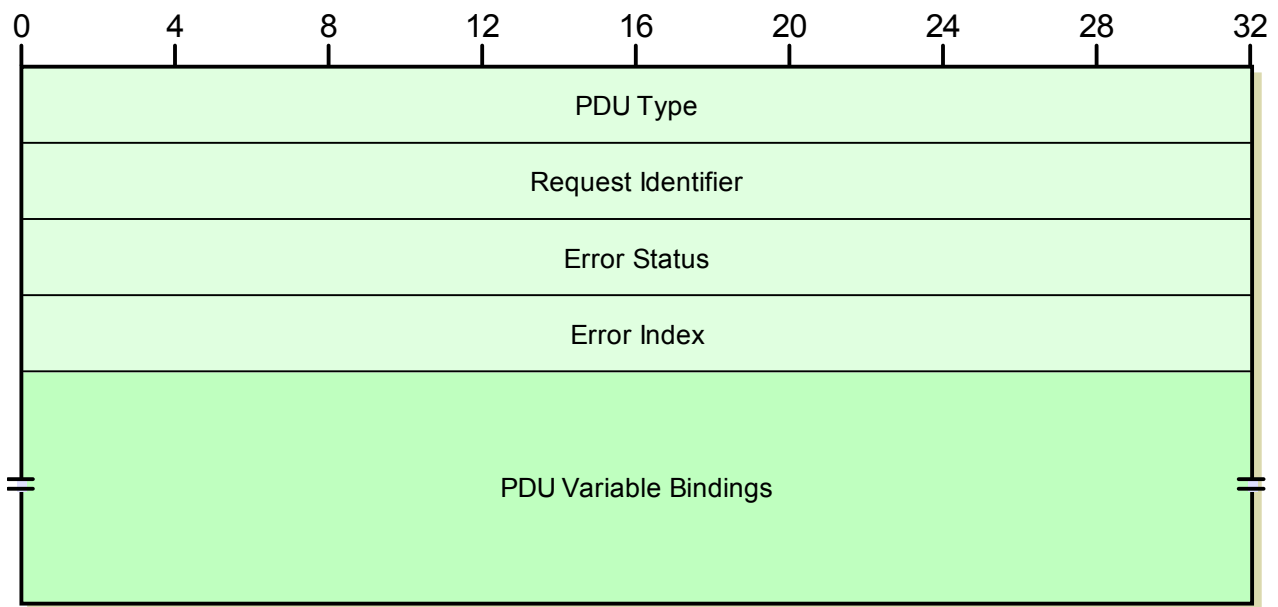
Figure 278: SNMP Version 1 (SNMPv1) Common PDU Format
