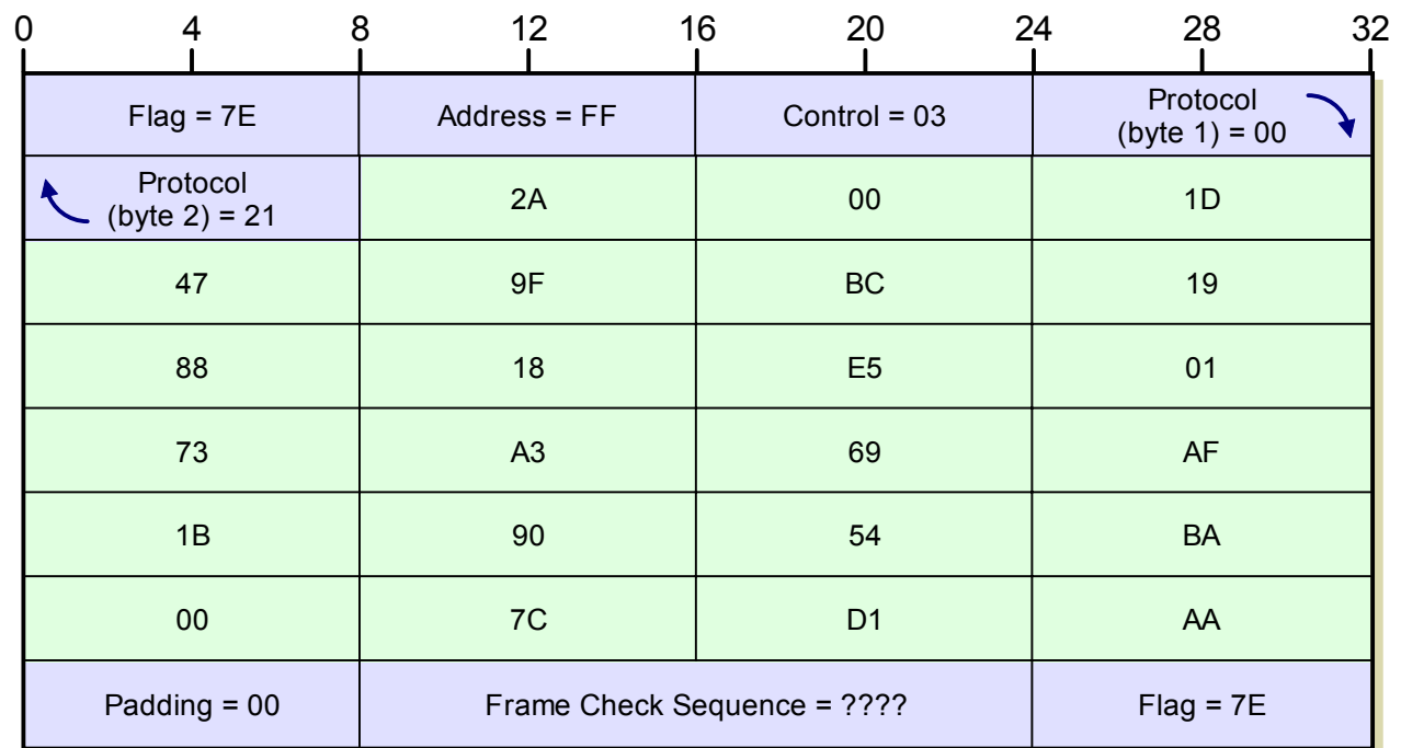
Figure 33: Sample PPP Data Frame
