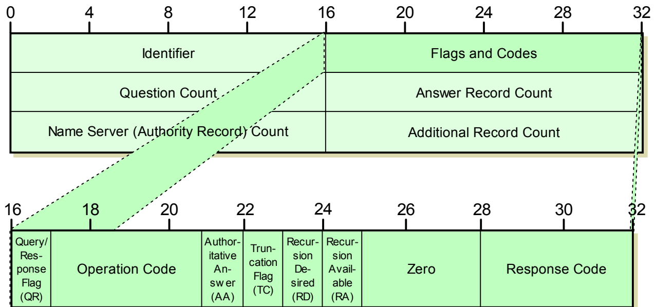
Figure 248: DNS Message Header Format
