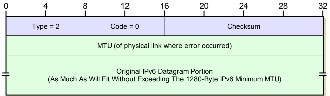
Figure 153: ICMPv6 Packet Too Big Message Format
