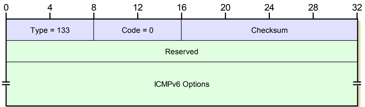
Figure 159: ICMPv6 Router Solicitation Message Format
