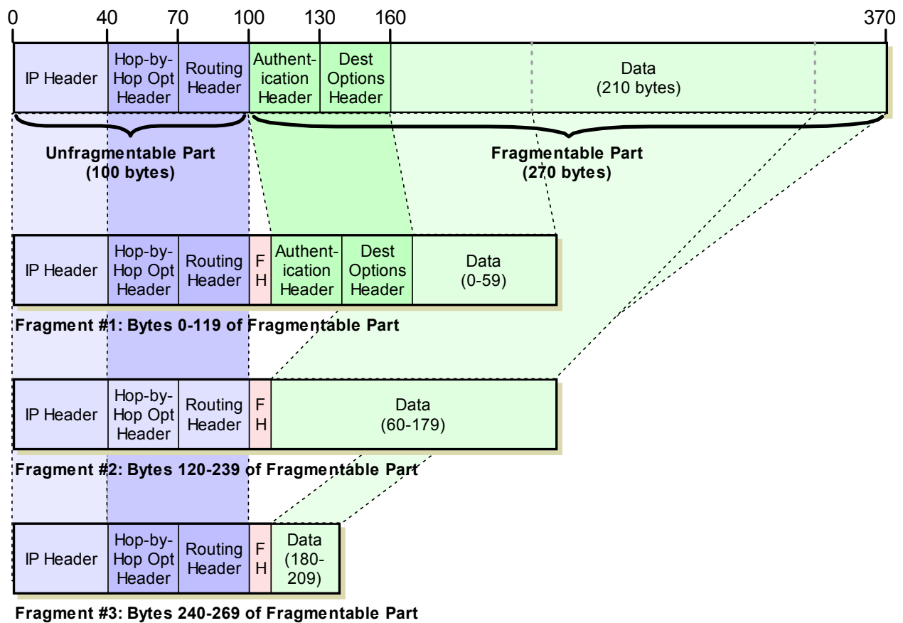
Figure 110: IPv6 Datagram Fragmentation
