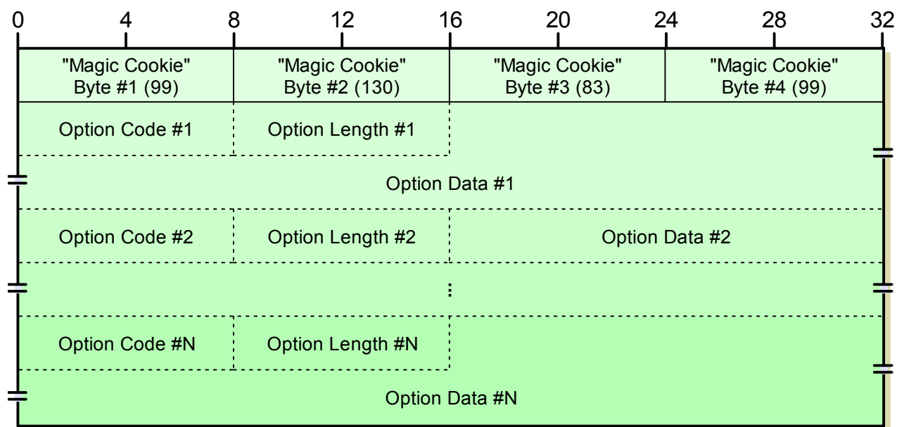
Figure 268: DHCP Options Field Format
