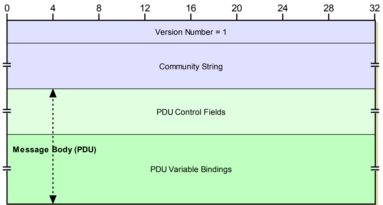
Figure 281: Community-Based SNMP Version 2 (SNMPv2c) General Message Format
