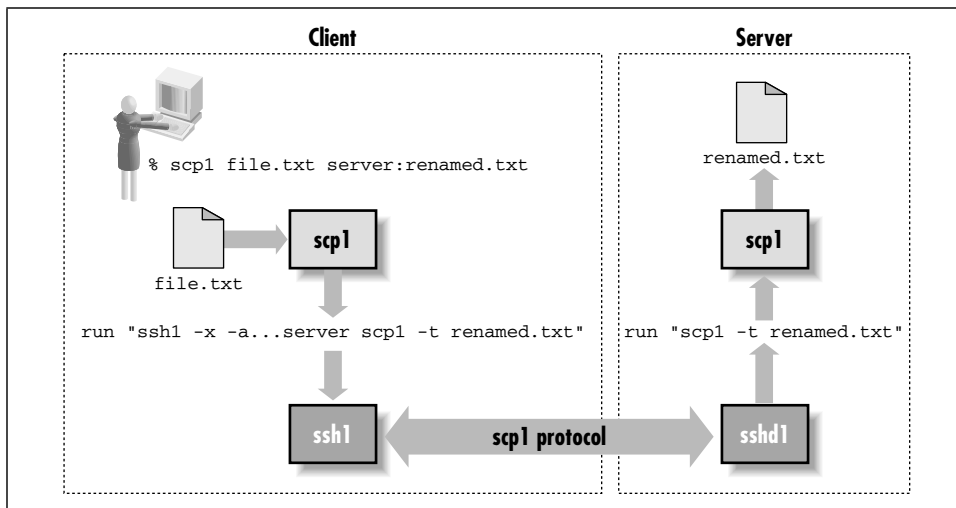
Figure 3-6. scp1 operation
