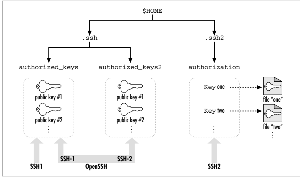
Figure 6-3. SSH authorization files (public keys) and the programs that use them
