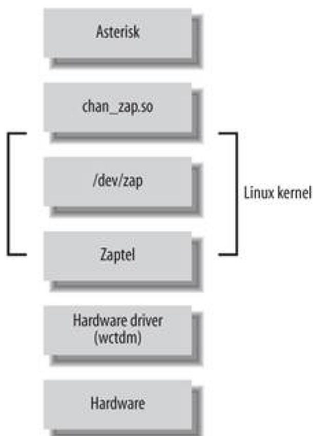
Figure 3-1. Layers of device interaction with Asterisk
