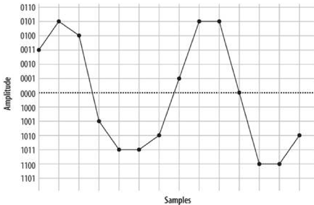
Figure 7-6. Delineated signal
