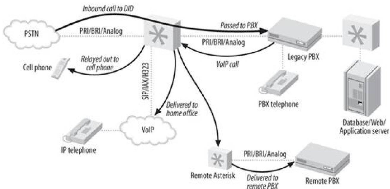
Figure 11-1. Asterisk as a PBX gateway
