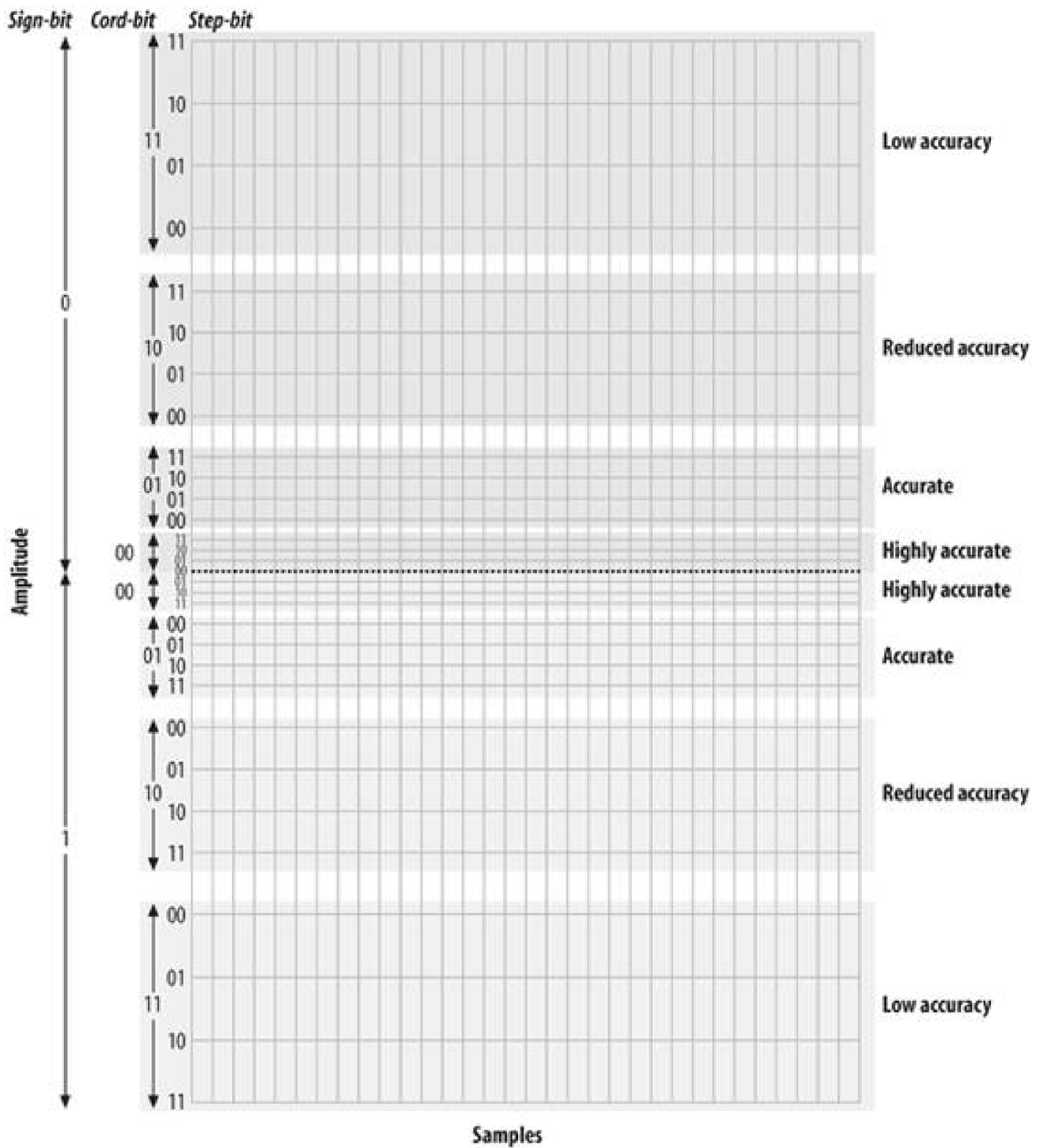
Figure 7-11. Five-bit companding
