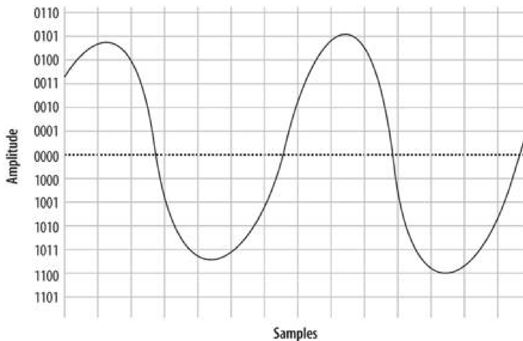
Figure 7-2. A simple sinusoidal (sine) wave
