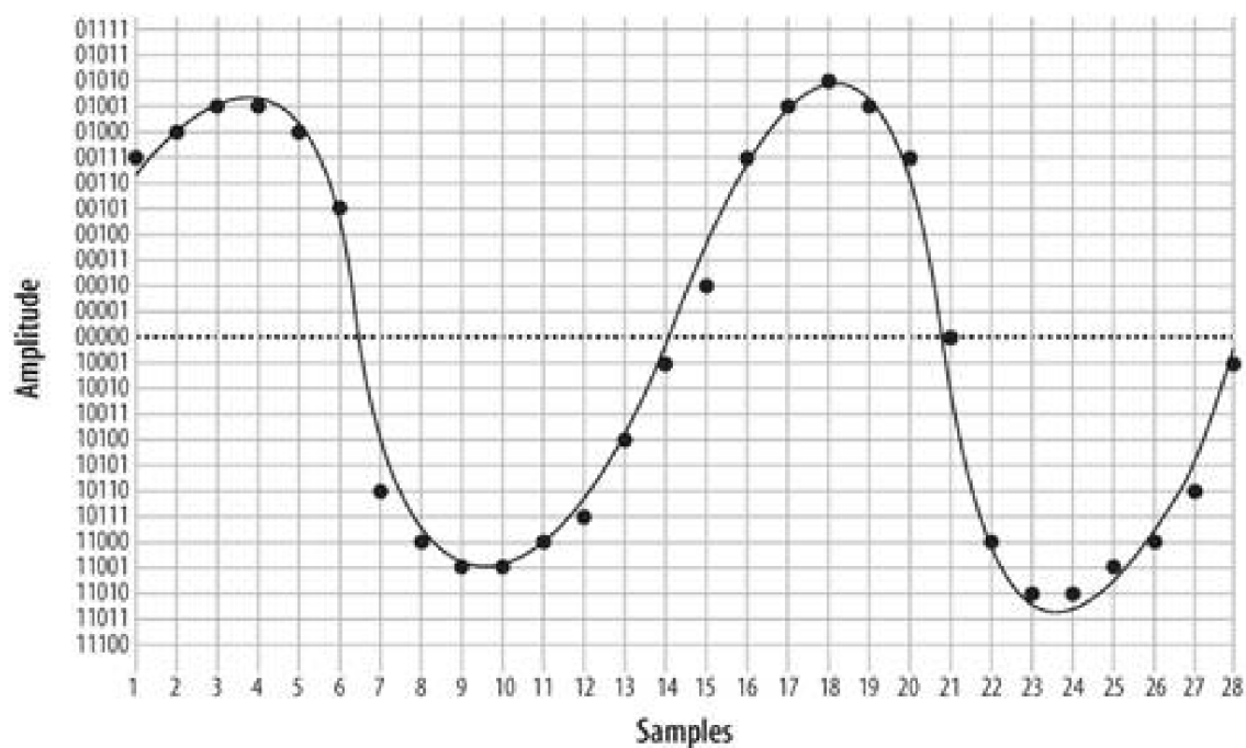
Figure 7-8. The same waveform at double the resolution
