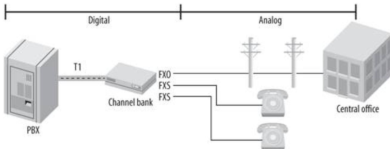
Figure 2-2. Channel bank
