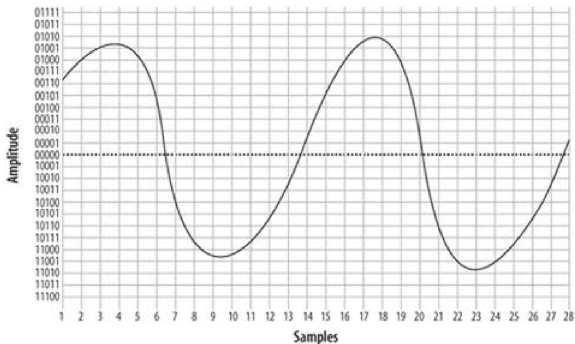
Figure 7-7. The same waveform, on a higher-resolution overlay
