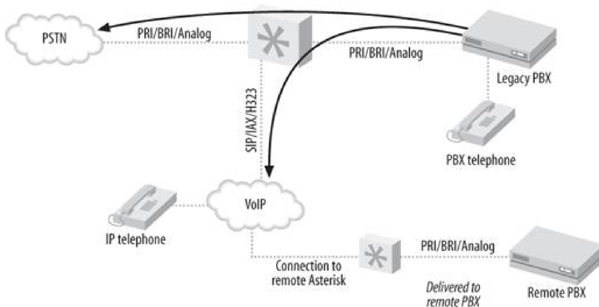
Figure 11-3. VoIP-enabling a legacy PBX
