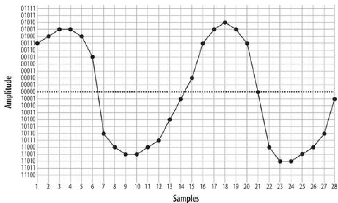
Figure 7-10. Waveform delineated from five-bit PCM
