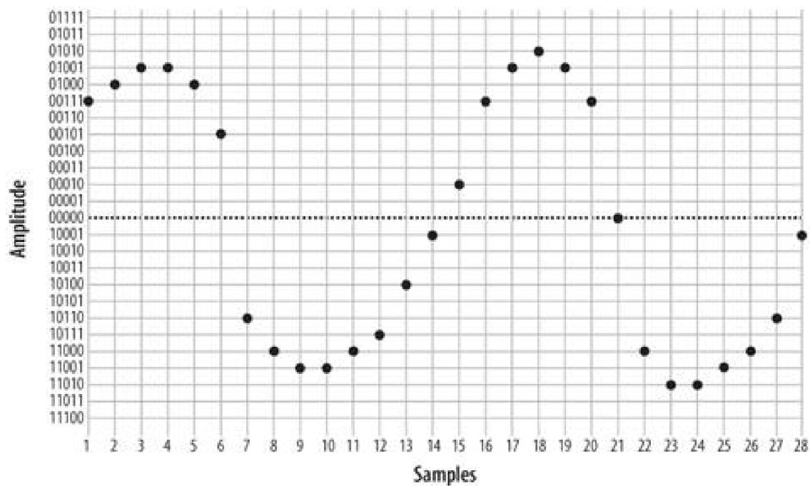
Figure 7-9. Five-bit plotted PCM signal
