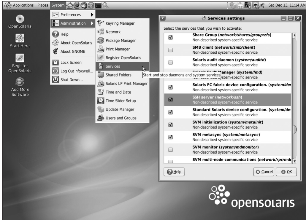
Figure 5-4. Using the Services GUI to select and disable the ssh service
