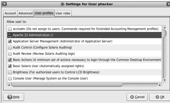
Figure 4-11. Setting a user's permission profile
