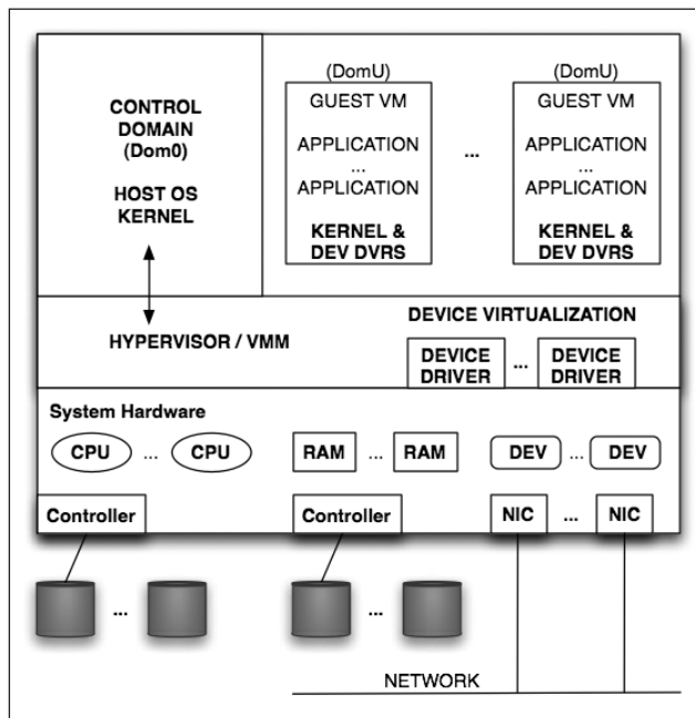
Figure 7-1. The Type 1 hypervisor architecture
