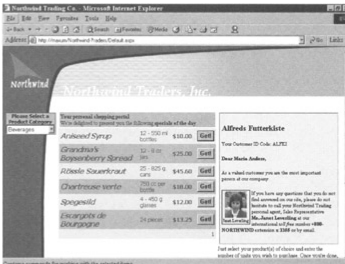
Figure 10.8: Login.aspx.
