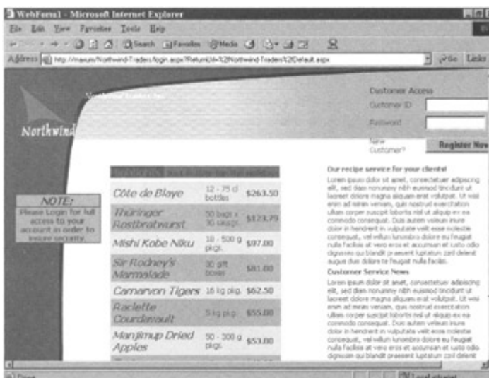
Figure 10.9: Checkout.aspx.
