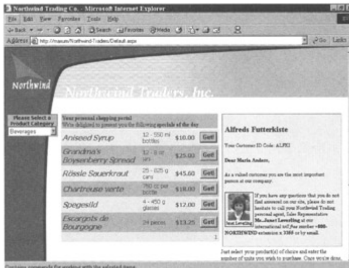
Figure 10.7: Default.aspx.
